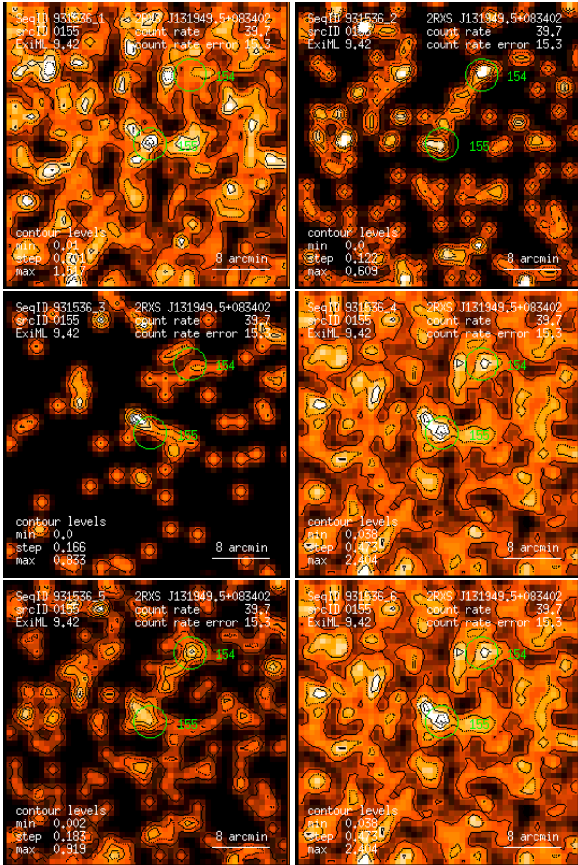
Figure 155: RASS 931536: detection 0155: band rate images, Gaussian filter: (1) PSPC channels 11 – 41, (2) 52 – 90, (3) 91 – 201, (4) 11 – 235, (5) 52 – 201, (6) 11 – 201. Broad band rates in counts/ks. Band rate contour levels in counts/ks/arcmin 2 .
