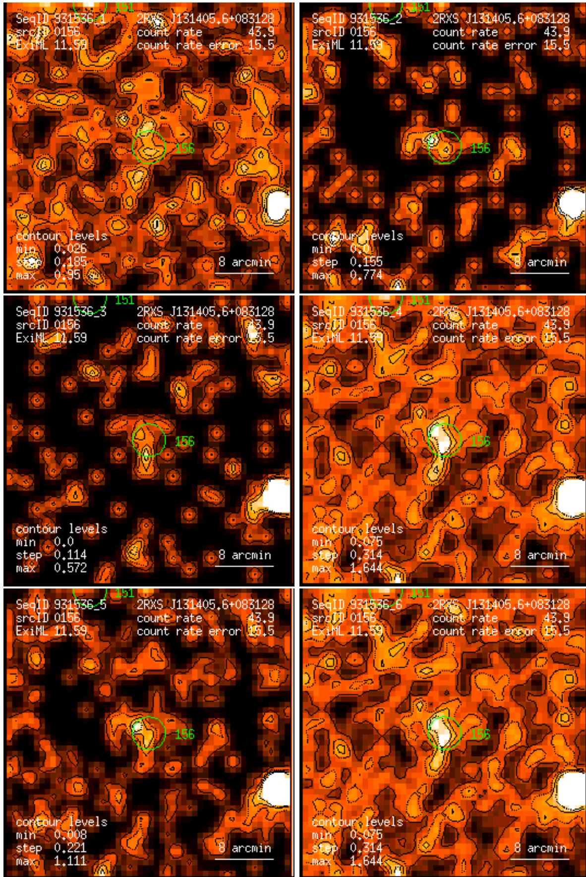
Figure 156: RASS 931536: detection 0156: band rate images, Gaussian filter: (1) PSPC channels 11 – 41, (2) 52 – 90, (3) 91 – 201, (4) 11 – 235, (5) 52 – 201, (6) 11 – 201. Broad band rates in counts/ks. Band rate contour levels in counts/ks/arcmin 2 .
