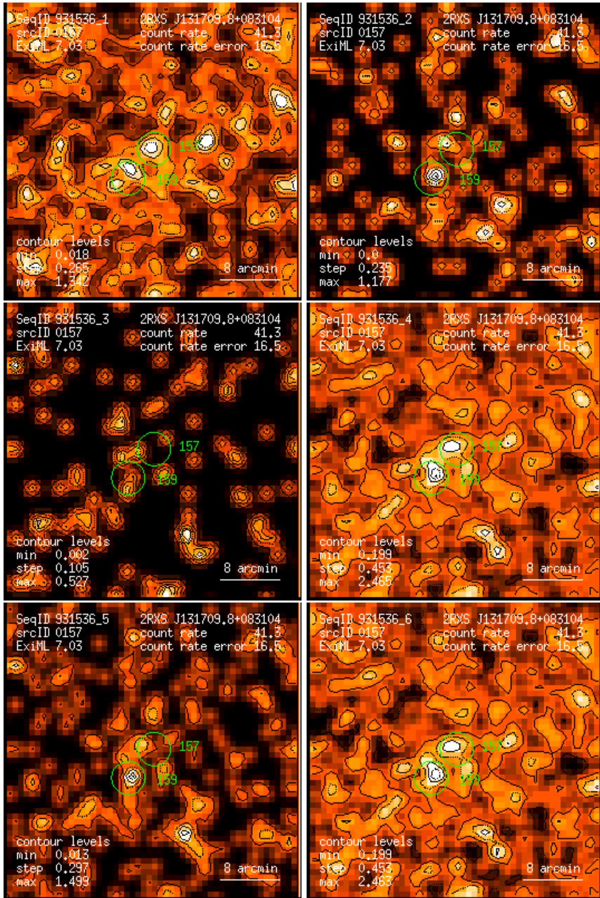
Figure 157: RASS 931536: detection 0157: band rate images, Gaussian filter: (1) PSPC channels 11 – 41, (2) 52 – 90, (3) 91 – 201, (4) 11 – 235, (5) 52 – 201, (6) 11 – 201. Broad band rates in counts/ks. Band rate contour levels in counts/ks/arcmin 2 .
