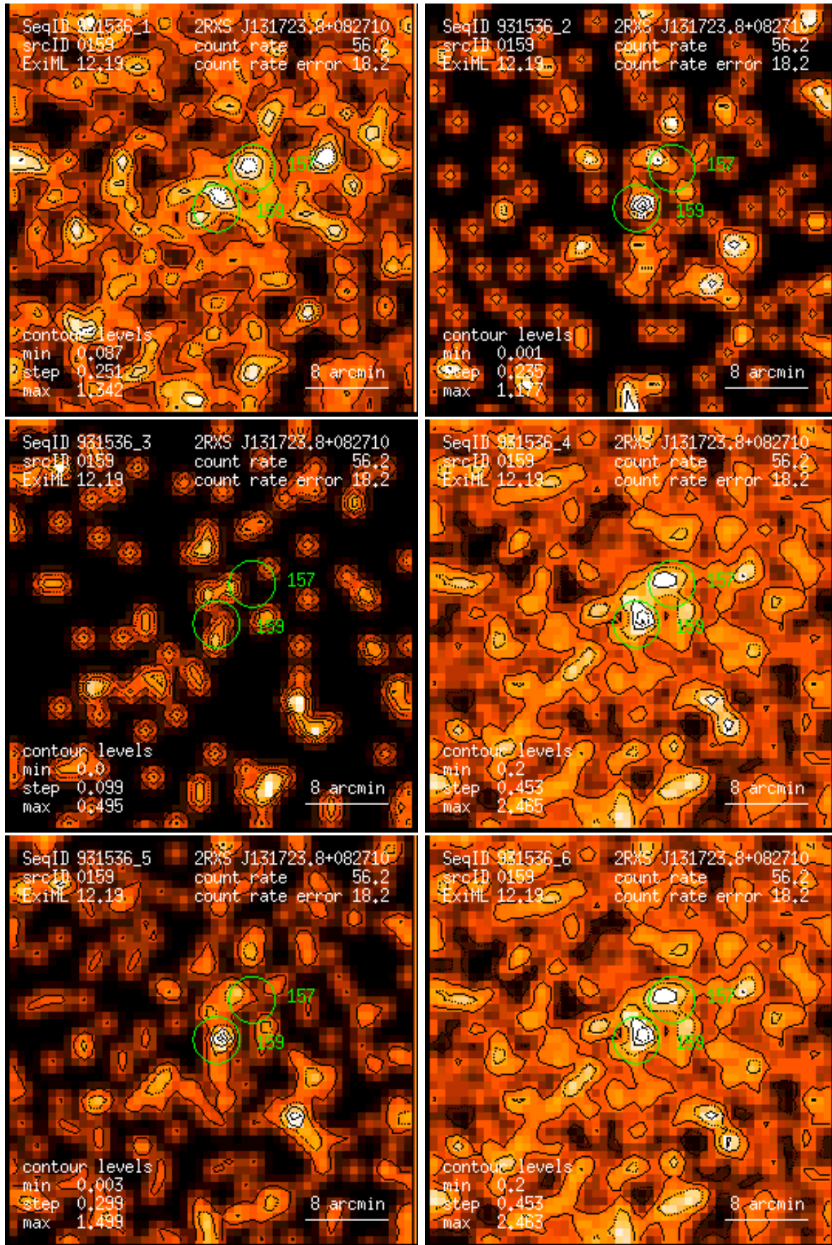
Figure 159: RASS 931536: detection 0159: band rate images, Gaussian filter: (1) PSPC channels 11 – 41, (2) 52 – 90, (3) 91 – 201, (4) 11 – 235, (5) 52 – 201, (6) 11 – 201. Broad band rates in counts/ks. Band rate contour levels in counts/ks/arcmin 2 .
