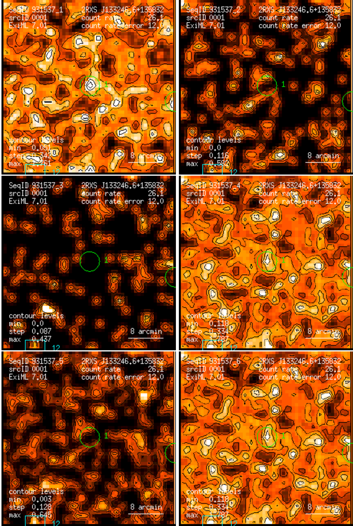
Figure 1: RASS 931537: detection 0001: band rate images, Gaussian filter: (1) PSPC channels 11 – 41, (2) 52 – 90, (3) 91 – 201, (4) 11 – 235, (5) 52 – 201, (6) 11 – 201. Broad band rates in counts/ks. Band rate contour levels in counts/ks/arcmin 2 .
