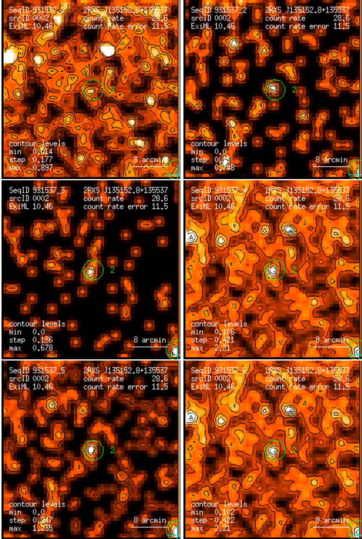
Figure 2: RASS 931537: detection 0002: band rate images, Gaussian filter: (1) PSPC channels 11 – 41, (2) 52 – 90, (3) 91 – 201, (4) 11 – 235, (5) 52 – 201, (6) 11 – 201. Broad band rates in counts/ks. Band rate contour levels in counts/ks/arcmin 2 .
