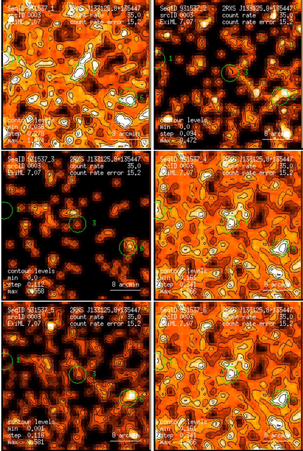
Figure 3: RASS 931537: detection 0003: band rate images, Gaussian filter: (1) PSPC channels 11 – 41, (2) 52 – 90, (3) 91 – 201, (4) 11 – 235, (5) 52 – 201, (6) 11 – 201. Broad band rates in counts/ks. Band rate contour levels in counts/ks/arcmin 2 .
