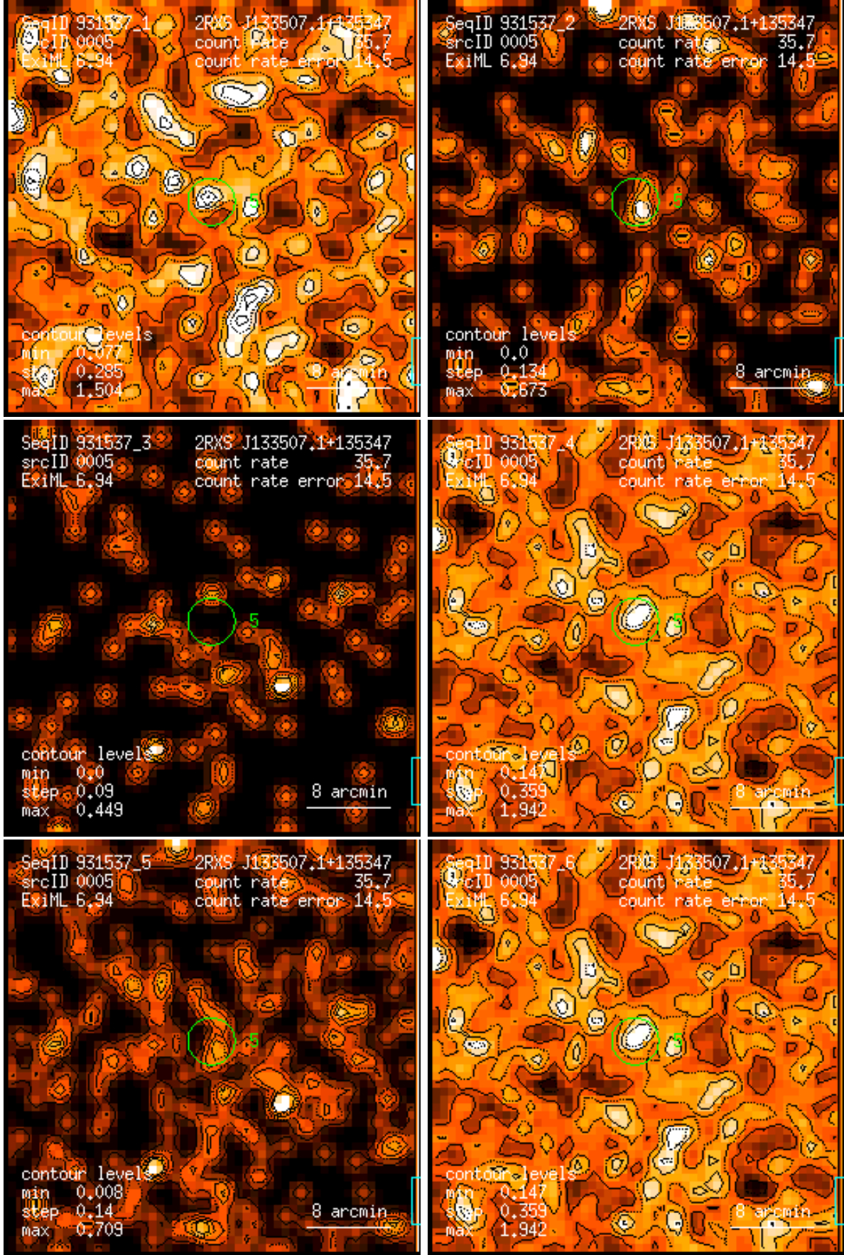
Figure 5: RASS 931537: detection 0005: band rate images, Gaussian filter: (1) PSPC channels 11 – 41, (2) 52 – 90, (3) 91 – 201, (4) 11 – 235, (5) 52 – 201, (6) 11 – 201. Broad band rates in counts/ks. Band rate contour levels in counts/ks/arcmin 2 .
