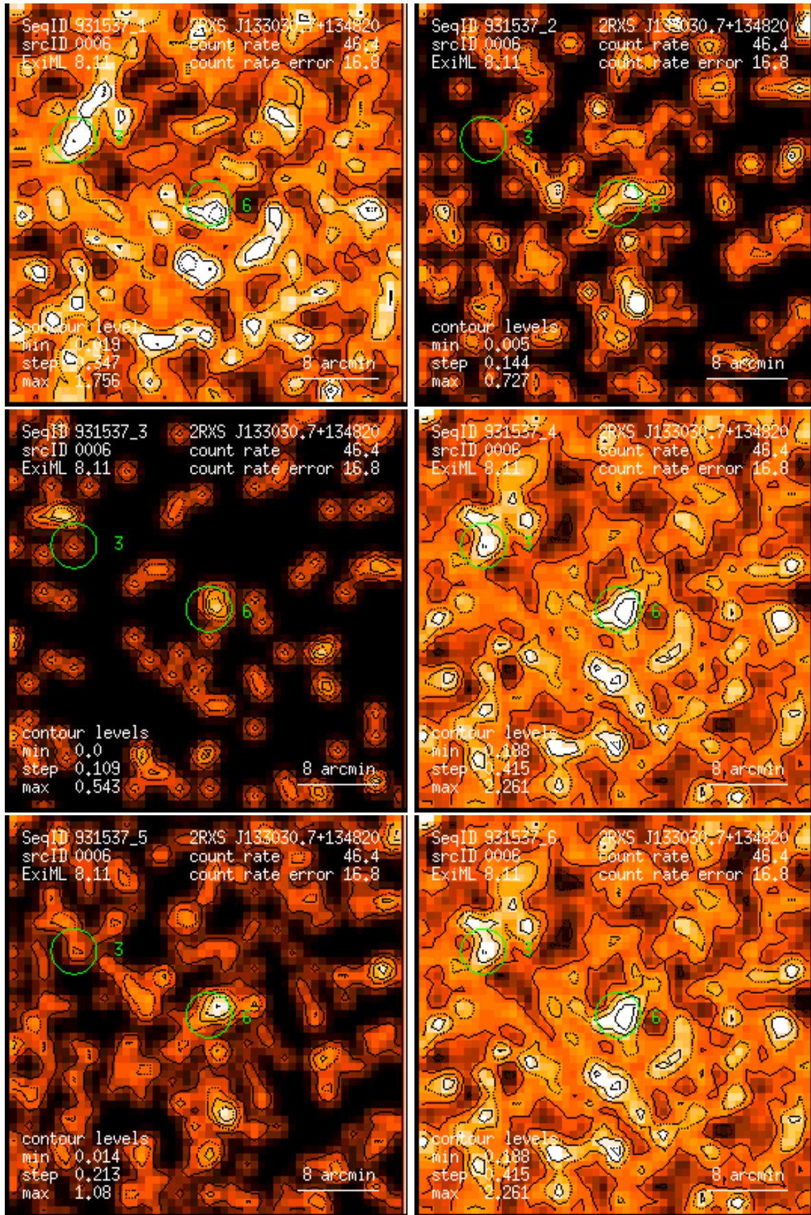
Figure 6: RASS 931537: detection 0006: band rate images, Gaussian filter: (1) PSPC channels 11 – 41, (2) 52 – 90, (3) 91 – 201, (4) 11 – 235, (5) 52 – 201, (6) 11 – 201. Broad band rates in counts/ks. Band rate contour levels in counts/ks/arcmin 2 .
