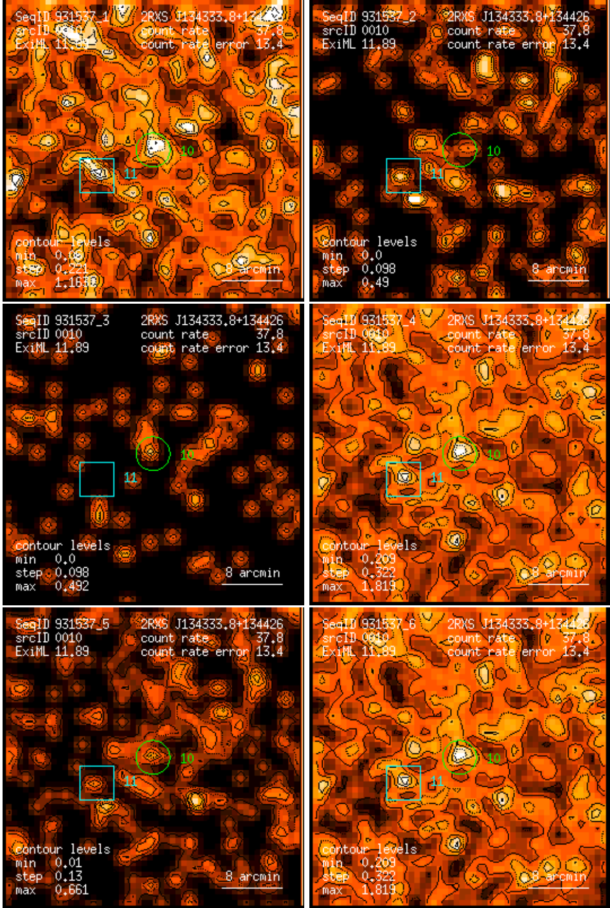
Figure 10: RASS 931537: detection 0010: band rate images, Gaussian filter: (1) PSPC channels 11 – 41, (2) 52 – 90, (3) 91 – 201, (4) 11 – 235, (5) 52 – 201, (6) 11 – 201. Broad band rates in counts/ks. Band rate contour levels in counts/ks/arcmin 2 .
