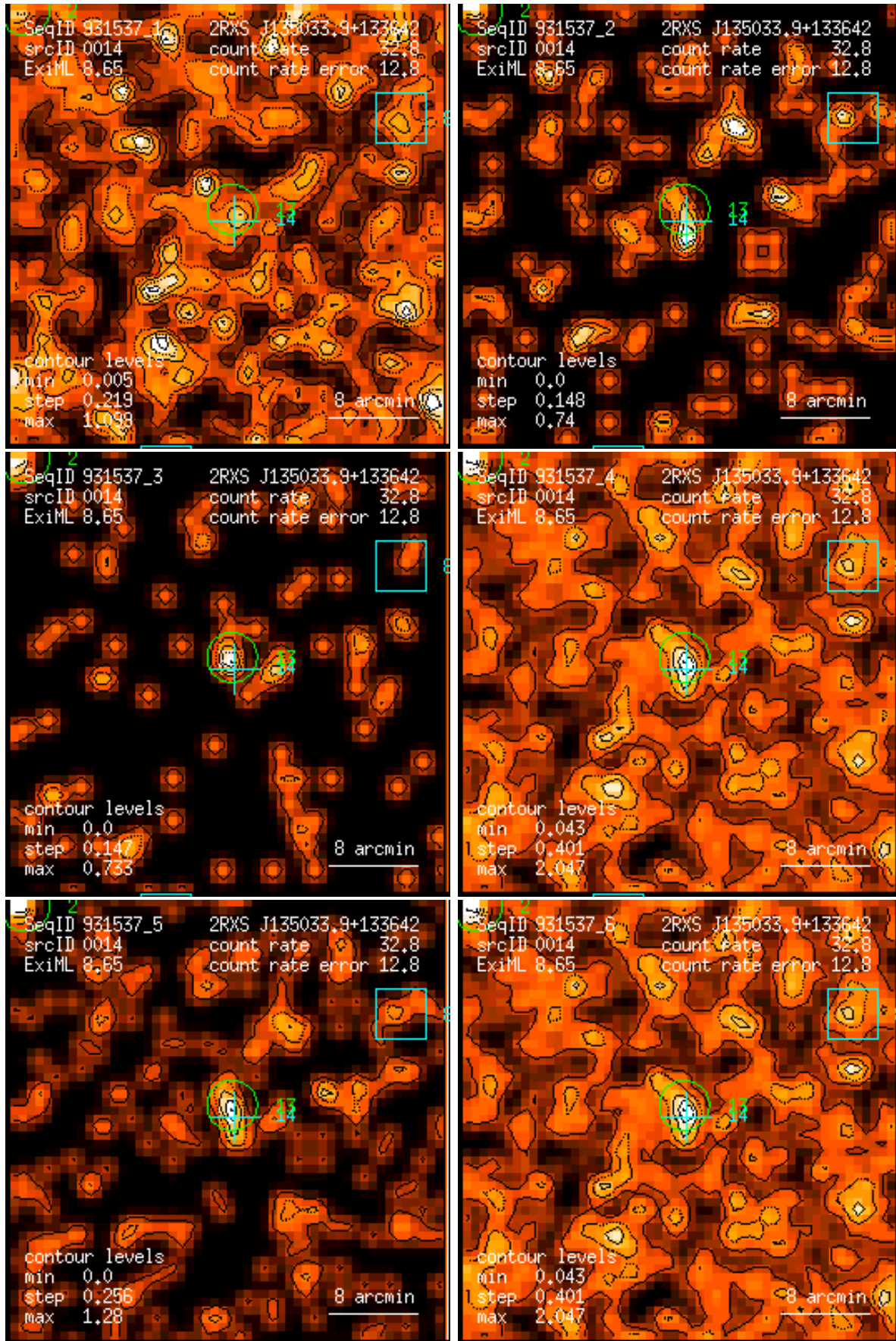
Figure 14: RASS 931537: detection 0014: band rate images, Gaussian filter: (1) PSPC channels 11 – 41, (2) 52 – 90, (3) 91 – 201, (4) 11 – 235, (5) 52 – 201, (6) 11 – 201. Broad band rates in counts/ks. Band rate contour levels in counts/ks/arcmin 2 .
