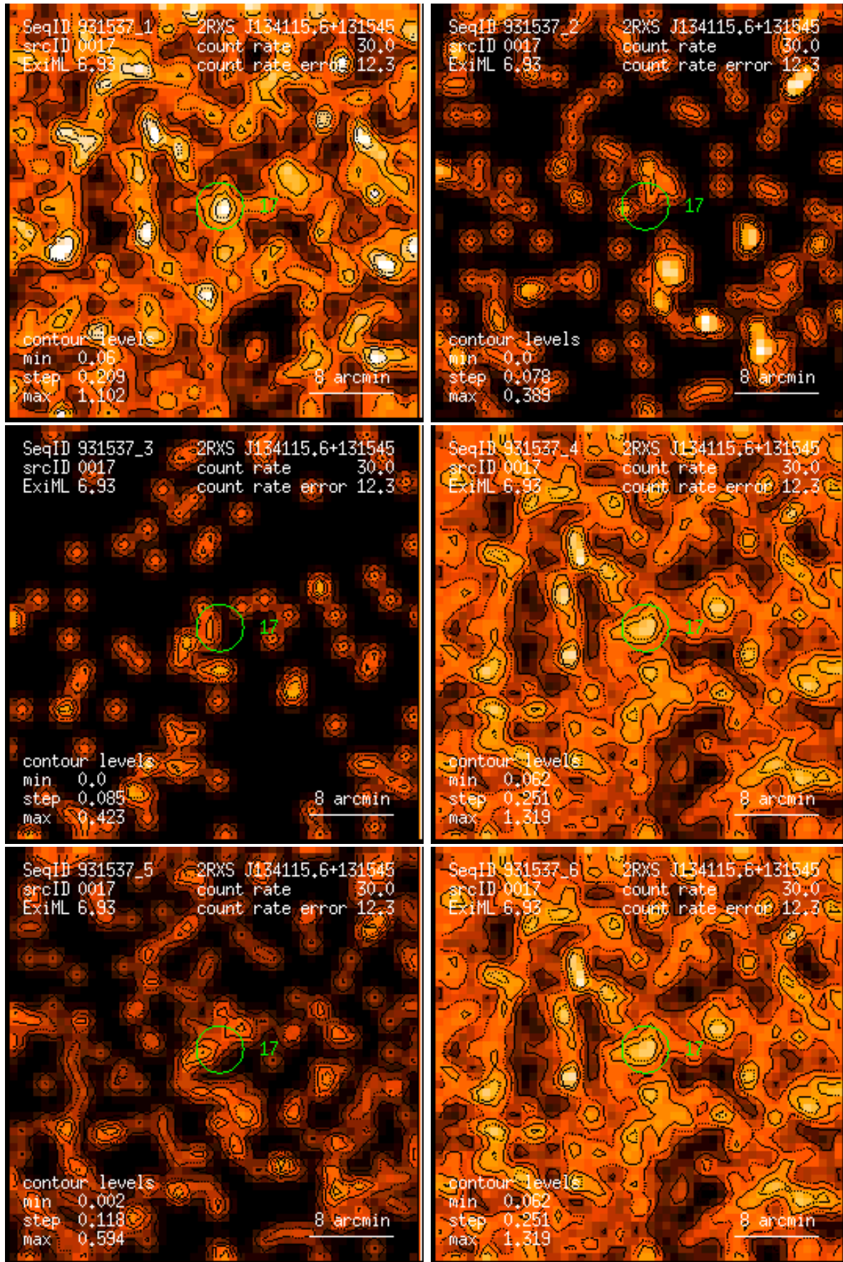
Figure 17: RASS 931537: detection 0017: band rate images, Gaussian filter: (1) PSPC channels 11 – 41, (2) 52 – 90, (3) 91 – 201, (4) 11 – 235, (5) 52 – 201, (6) 11 – 201. Broad band rates in counts/ks. Band rate contour levels in counts/ks/arcmin 2 .
