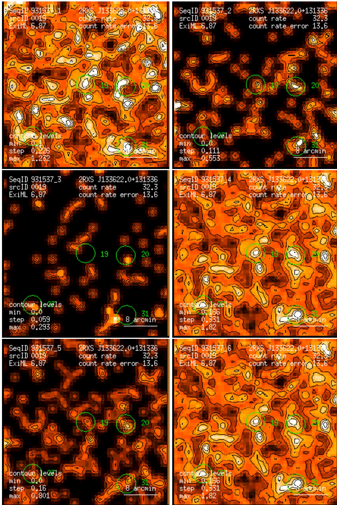
Figure 19: RASS 931537: detection 0019: band rate images, Gaussian filter: (1) PSPC channels 11 – 41, (2) 52 – 90, (3) 91 – 201, (4) 11 – 235, (5) 52 – 201, (6) 11 – 201. Broad band rates in counts/ks. Band rate contour levels in counts/ks/arcmin 2 .
