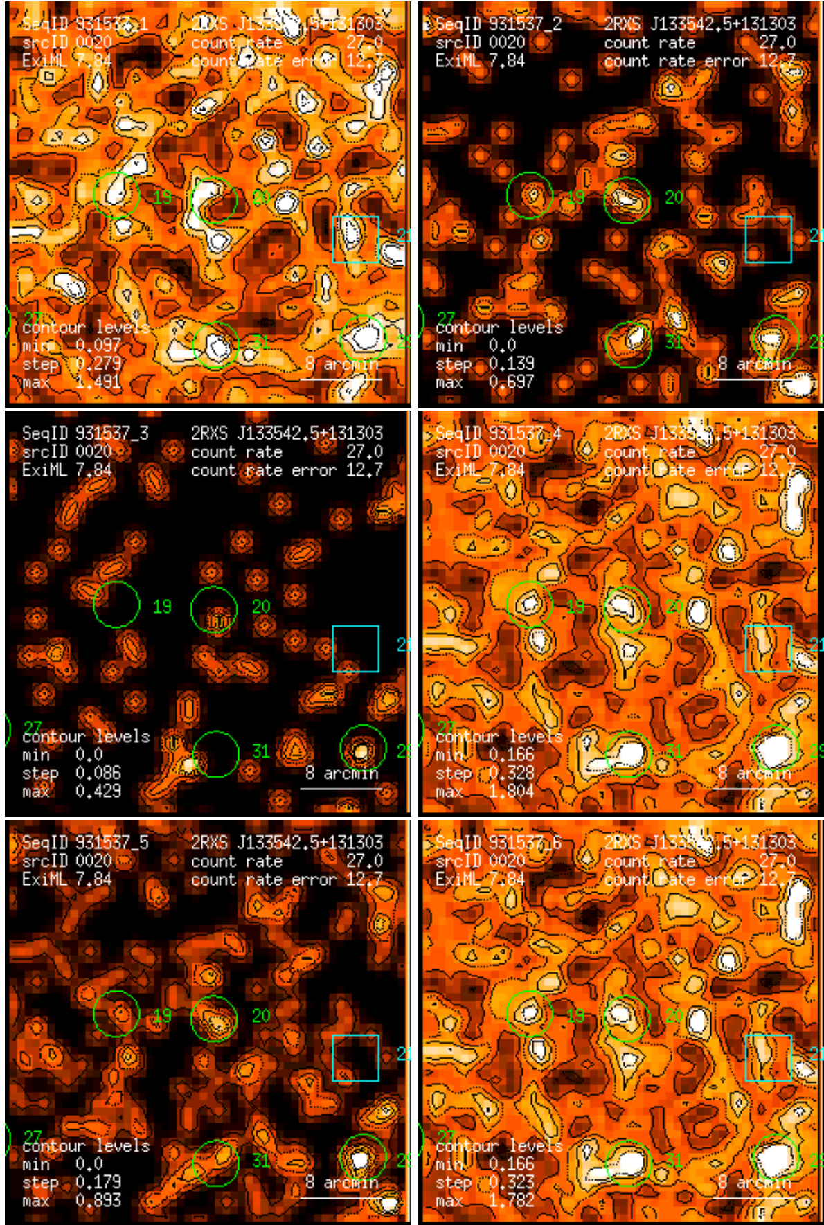
Figure 20: RASS 931537: detection 0020: band rate images, Gaussian filter: (1) PSPC channels 11 – 41, (2) 52 – 90, (3) 91 – 201, (4) 11 – 235, (5) 52 – 201, (6) 11 – 201. Broad band rates in counts/ks. Band rate contour levels in counts/ks/arcmin 2 .
