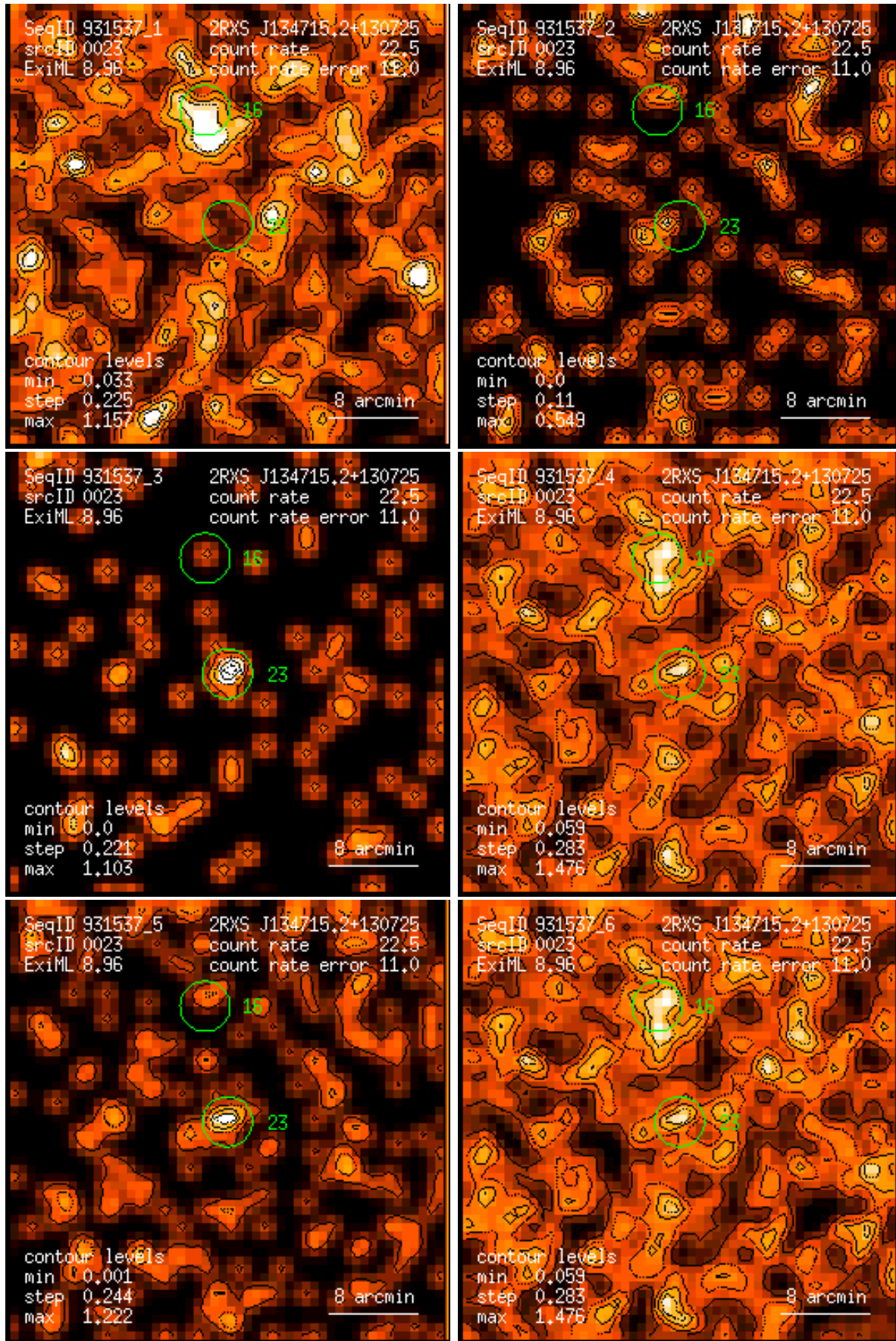
Figure 23: RASS 931537: detection 0023: band rate images, Gaussian filter: (1) PSPC channels 11 – 41, (2) 52 – 90, (3) 91 – 201, (4) 11 – 235, (5) 52 – 201, (6) 11 – 201. Broad band rates in counts/ks. Band rate contour levels in counts/ks/arcmin 2 .
