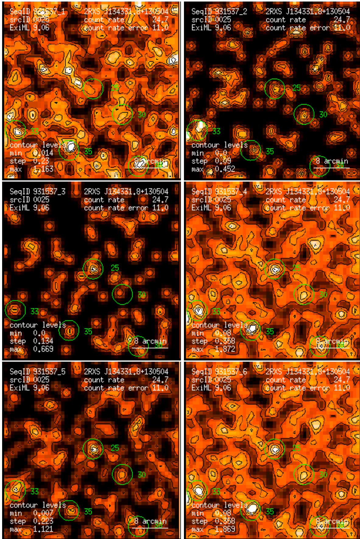
Figure 25: RASS 931537: detection 0025: band rate images, Gaussian filter: (1) PSPC channels 11 – 41, (2) 52 – 90, (3) 91 – 201, (4) 11 – 235, (5) 52 – 201, (6) 11 – 201. Broad band rates in counts/ks. Band rate contour levels in counts/ks/arcmin 2 .
