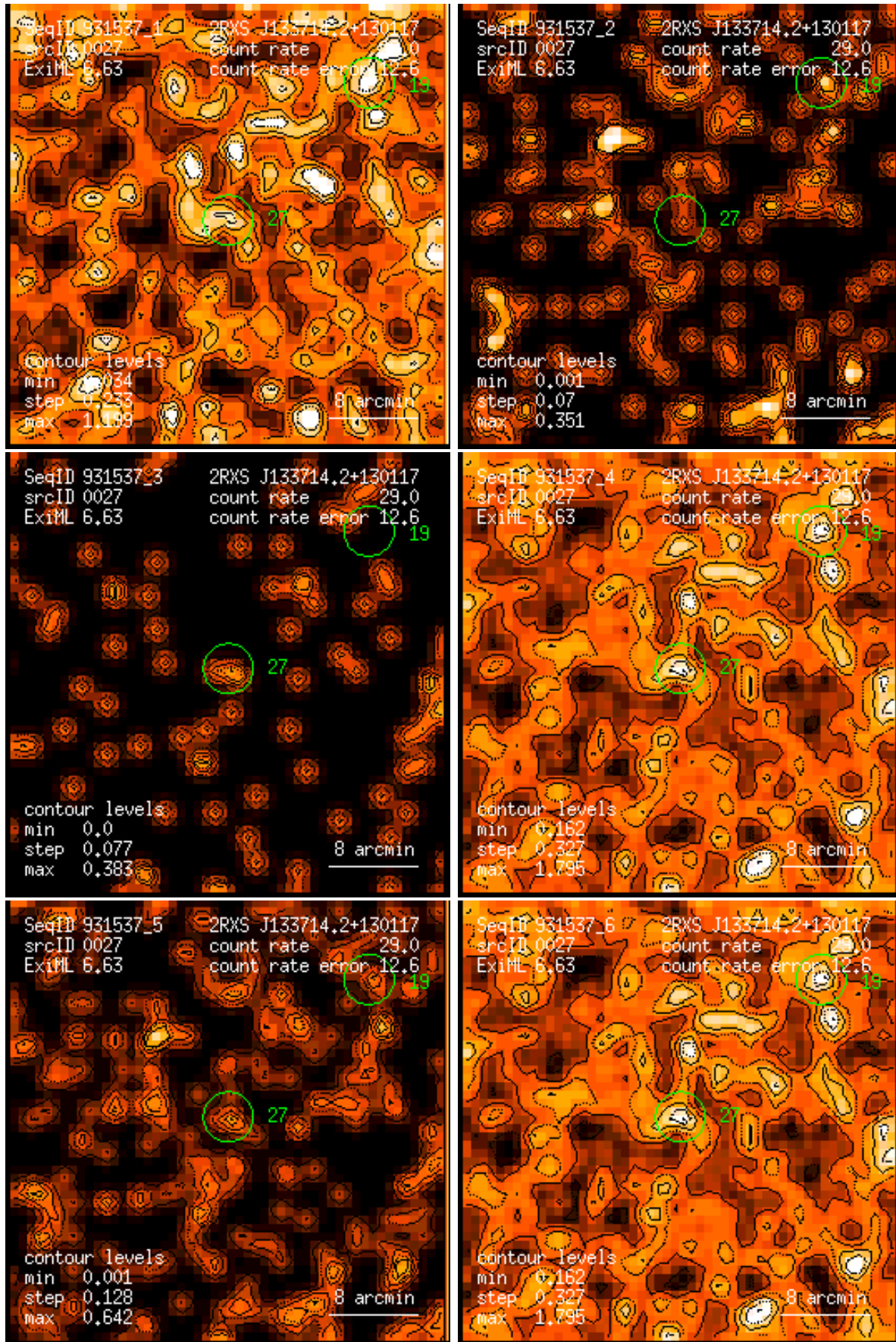
Figure 27: RASS 931537: detection 0027: band rate images, Gaussian filter: (1) PSPC channels 11 – 41, (2) 52 – 90, (3) 91 – 201, (4) 11 – 235, (5) 52 – 201, (6) 11 – 201. Broad band rates in counts/ks. Band rate contour levels in counts/ks/arcmin 2 .
