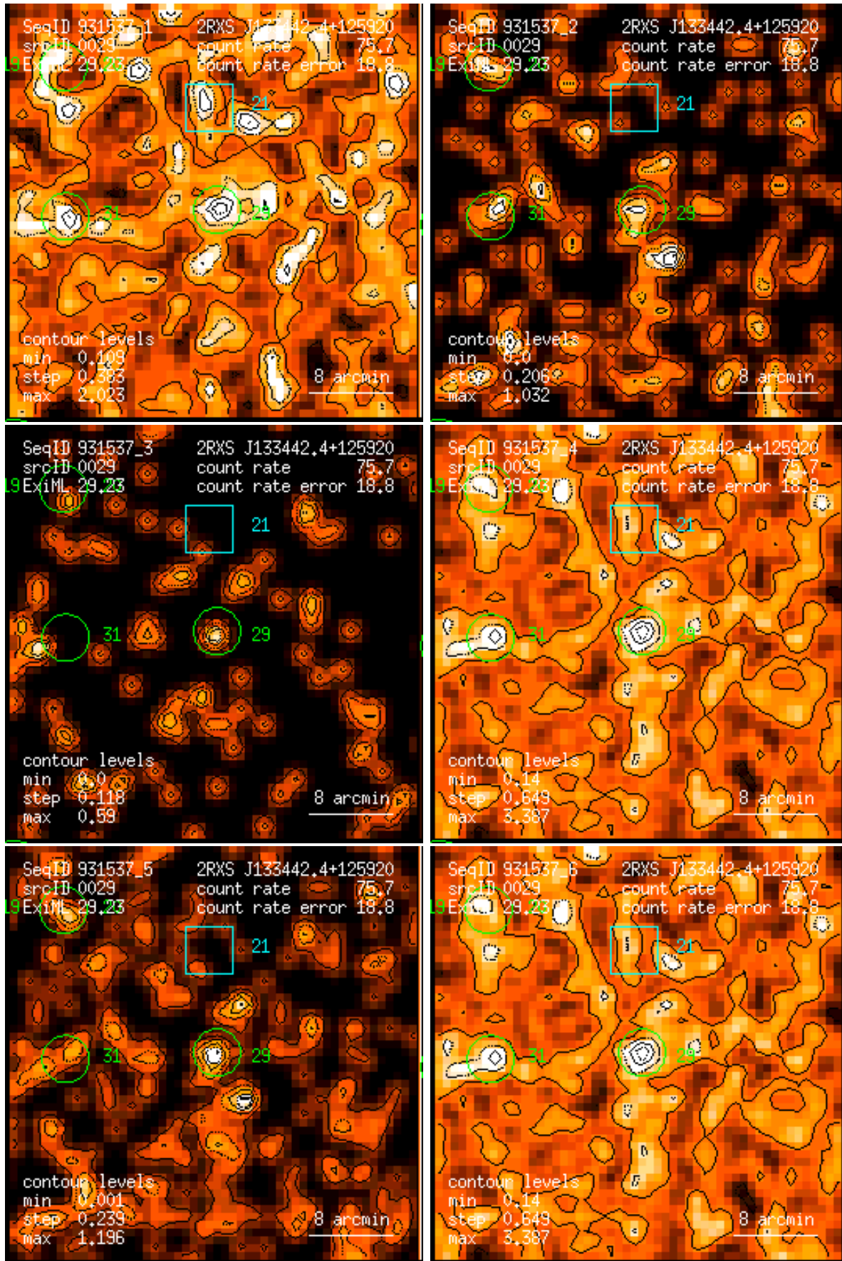
Figure 29: RASS 931537: detection 0029: band rate images, Gaussian filter: (1) PSPC channels 11 – 41, (2) 52 – 90, (3) 91 – 201, (4) 11 – 235, (5) 52 – 201, (6) 11 – 201. Broad band rates in counts/ks. Band rate contour levels in counts/ks/arcmin 2 .
