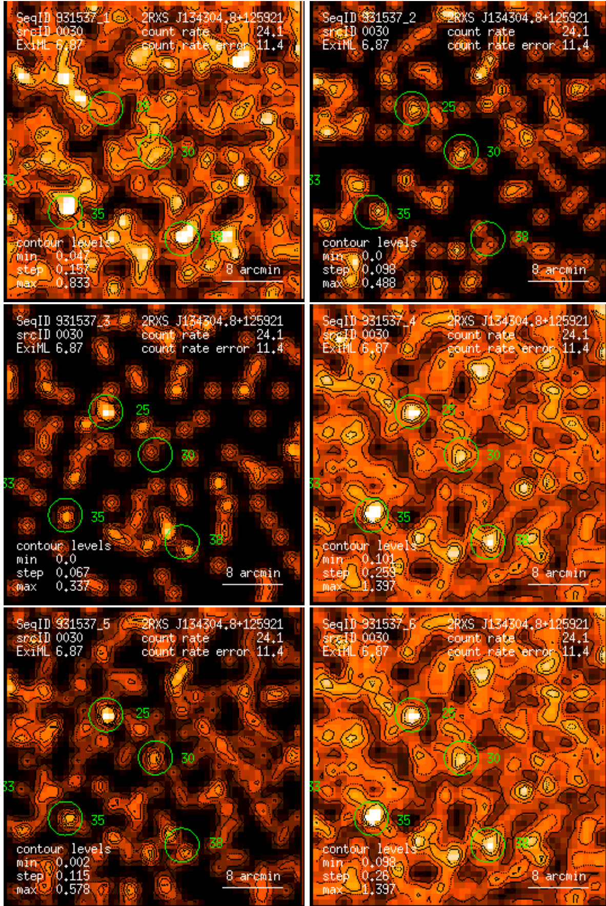
Figure 30: RASS 931537: detection 0030: band rate images, Gaussian filter: (1) PSPC channels 11 – 41, (2) 52 – 90, (3) 91 – 201, (4) 11 – 235, (5) 52 – 201, (6) 11 – 201. Broad band rates in counts/ks. Band rate contour levels in counts/ks/arcmin 2 .
