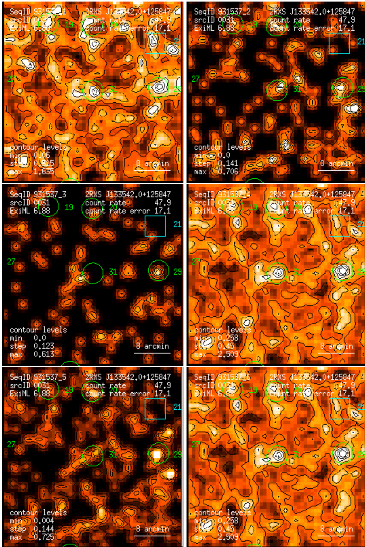
Figure 31: RASS 931537: detection 0031: band rate images, Gaussian filter: (1) PSPC channels 11 – 41, (2) 52 – 90, (3) 91 – 201, (4) 11 – 235, (5) 52 – 201, (6) 11 – 201. Broad band rates in counts/ks. Band rate contour levels in counts/ks/arcmin 2 .
