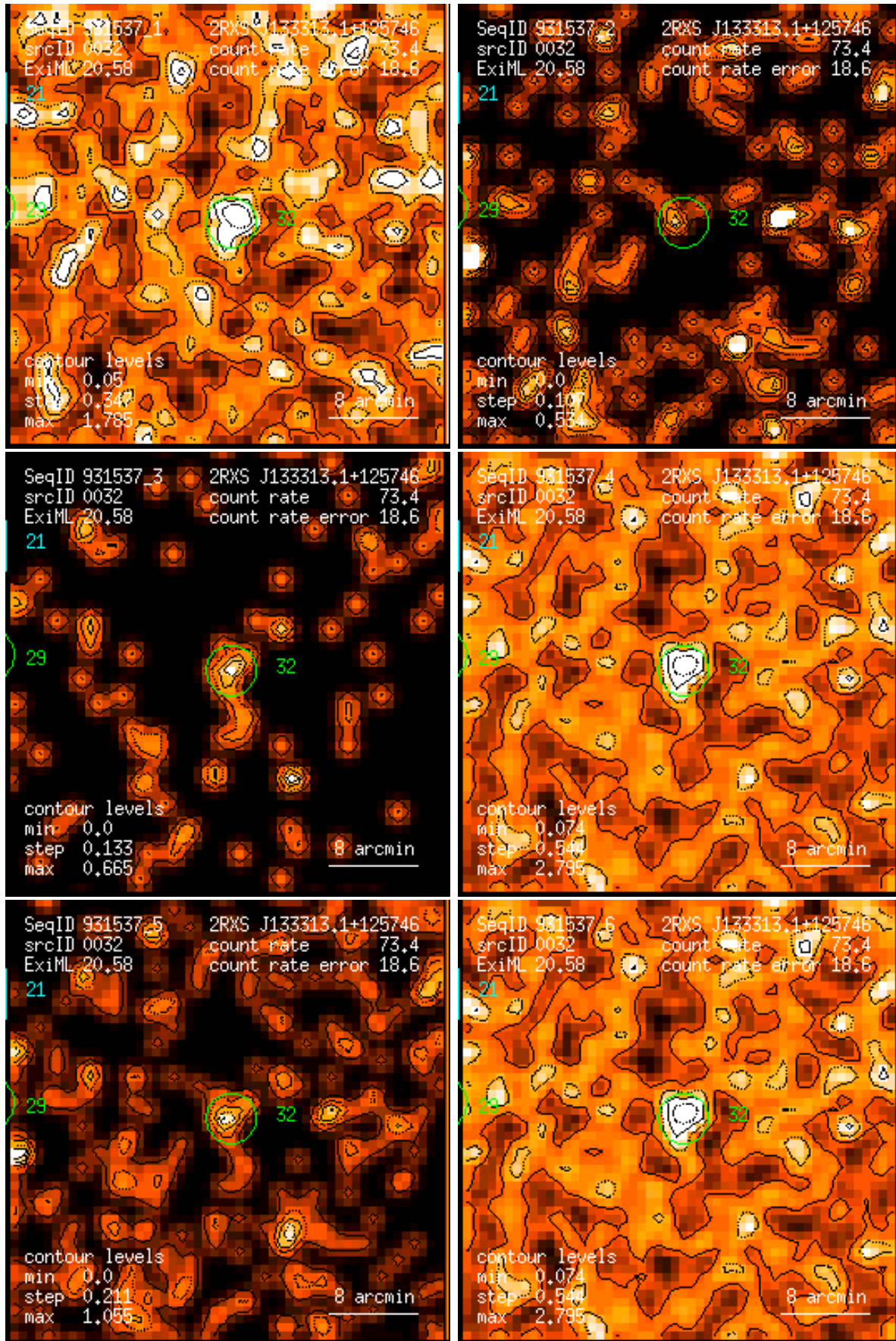
Figure 32: RASS 931537: detection 0032: band rate images, Gaussian filter: (1) PSPC channels 11 – 41, (2) 52 – 90, (3) 91 – 201, (4) 11 – 235, (5) 52 – 201, (6) 11 – 201. Broad band rates in counts/ks. Band rate contour levels in counts/ks/arcmin 2 .
