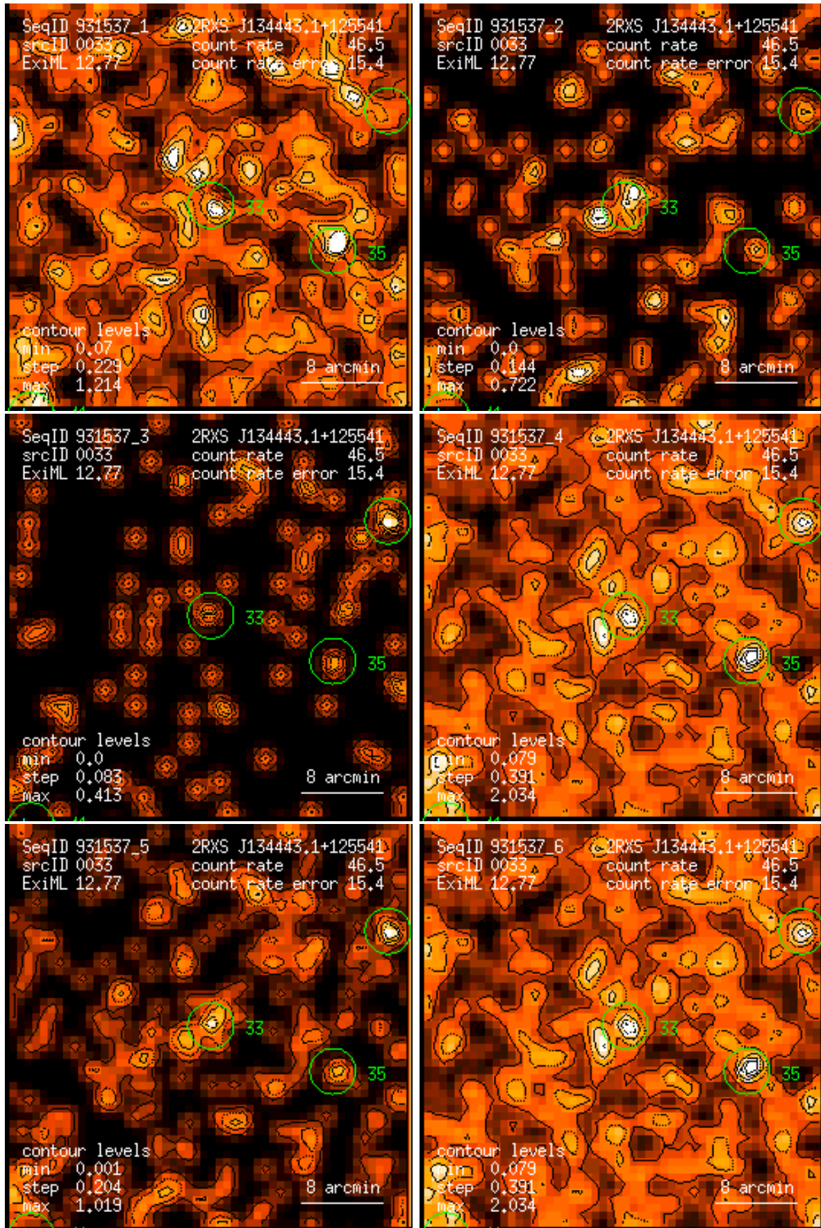
Figure 33: RASS 931537: detection 0033: band rate images, Gaussian filter: (1) PSPC channels 11 – 41, (2) 52 – 90, (3) 91 – 201, (4) 11 – 235, (5) 52 – 201, (6) 11 – 201. Broad band rates in counts/ks. Band rate contour levels in counts/ks/arcmin 2 .
