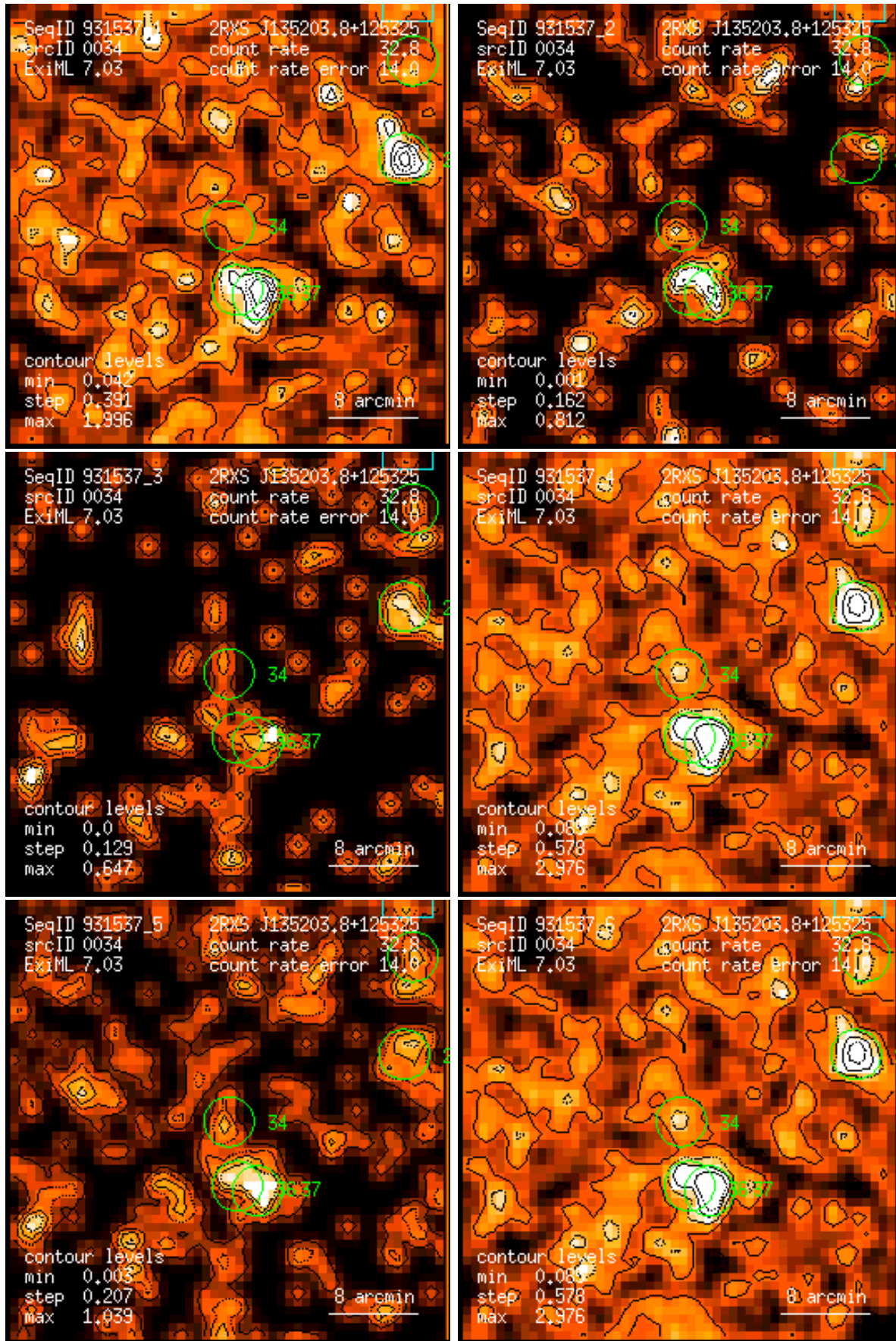
Figure 34: RASS 931537: detection 0034: band rate images, Gaussian filter: (1) PSPC channels 11 – 41, (2) 52 – 90, (3) 91 – 201, (4) 11 – 235, (5) 52 – 201, (6) 11 – 201. Broad band rates in counts/ks. Band rate contour levels in counts/ks/arcmin 2 .
