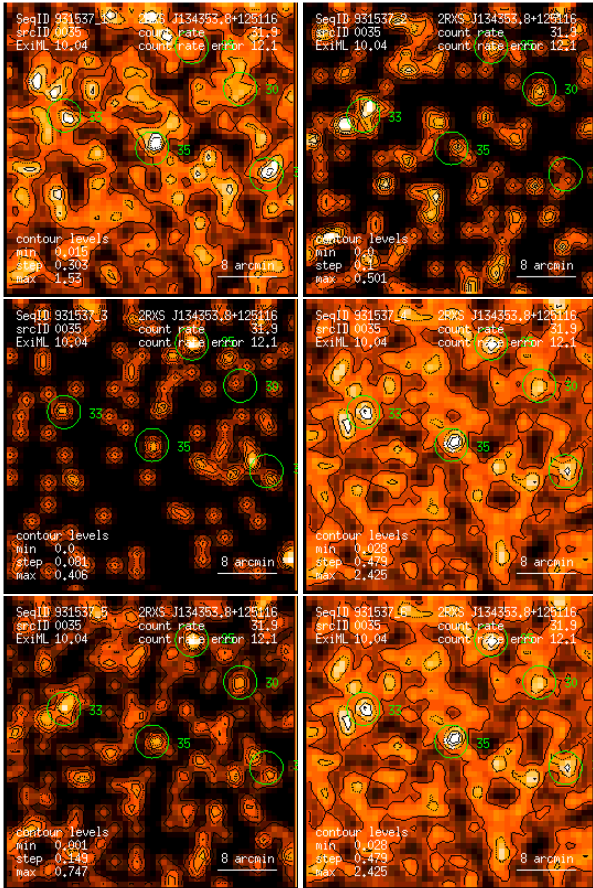
Figure 35: RASS 931537: detection 0035: band rate images, Gaussian filter: (1) PSPC channels 11 – 41, (2) 52 – 90, (3) 91 – 201, (4) 11 – 235, (5) 52 – 201, (6) 11 – 201. Broad band rates in counts/ks. Band rate contour levels in counts/ks/arcmin 2 .
