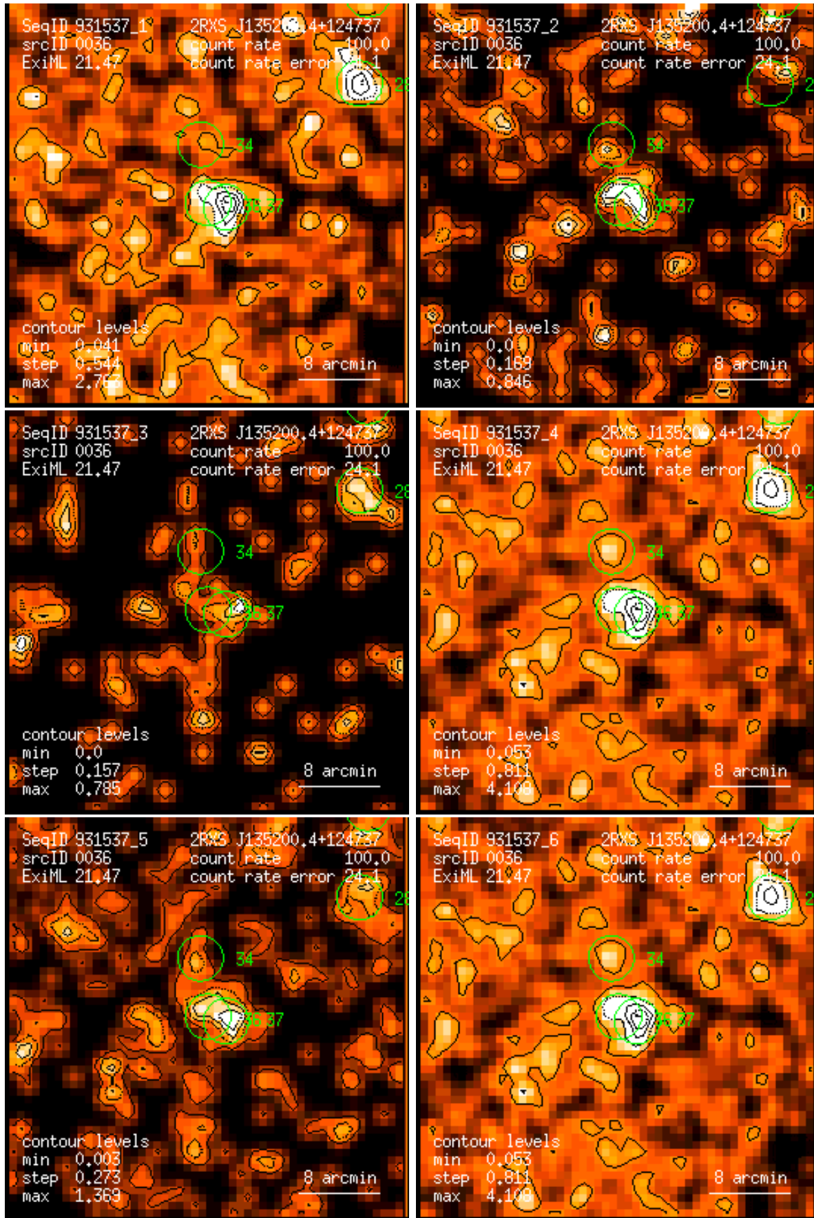
Figure 36: RASS 931537: detection 0036: band rate images, Gaussian filter: (1) PSPC channels 11 – 41, (2) 52 – 90, (3) 91 – 201, (4) 11 – 235, (5) 52 – 201, (6) 11 – 201. Broad band rates in counts/ks. Band rate contour levels in counts/ks/arcmin 2 .
