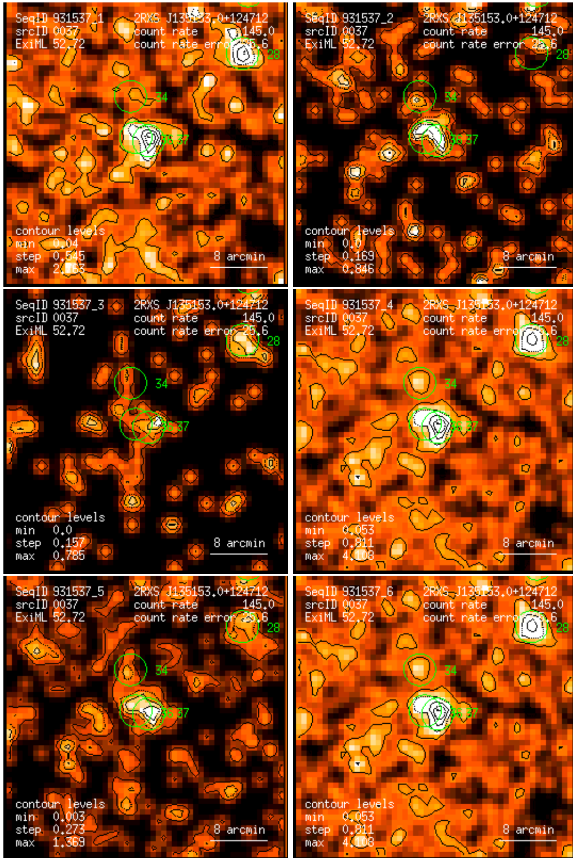
Figure 37: RASS 931537: detection 0037: band rate images, Gaussian filter: (1) PSPC channels 11 – 41, (2) 52 – 90, (3) 91 – 201, (4) 11 – 235, (5) 52 – 201, (6) 11 – 201. Broad band rates in counts/ks. Band rate contour levels in counts/ks/arcmin 2 .
