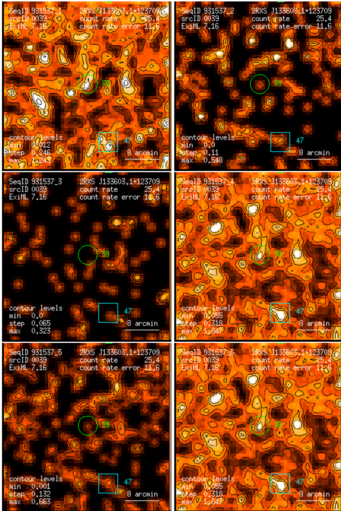
Figure 39: RASS 931537: detection 0039: band rate images, Gaussian filter: (1) PSPC channels 11 – 41, (2) 52 – 90, (3) 91 – 201, (4) 11 – 235, (5) 52 – 201, (6) 11 – 201. Broad band rates in counts/ks. Band rate contour levels in counts/ks/arcmin 2 .
