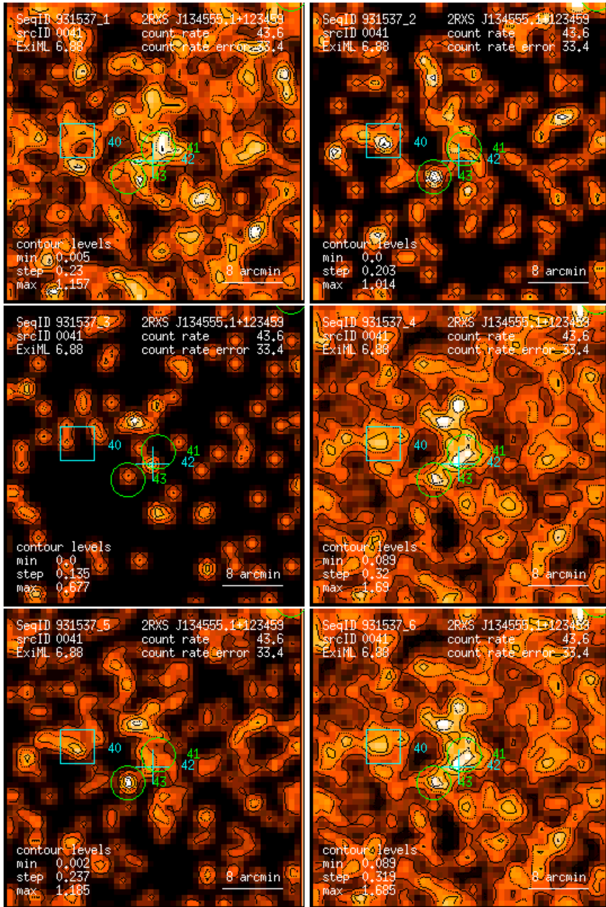
Figure 41: RASS 931537: detection 0041: band rate images, Gaussian filter: (1) PSPC channels 11 – 41, (2) 52 – 90, (3) 91 – 201, (4) 11 – 235, (5) 52 – 201, (6) 11 – 201. Broad band rates in counts/ks. Band rate contour levels in counts/ks/arcmin 2 .
