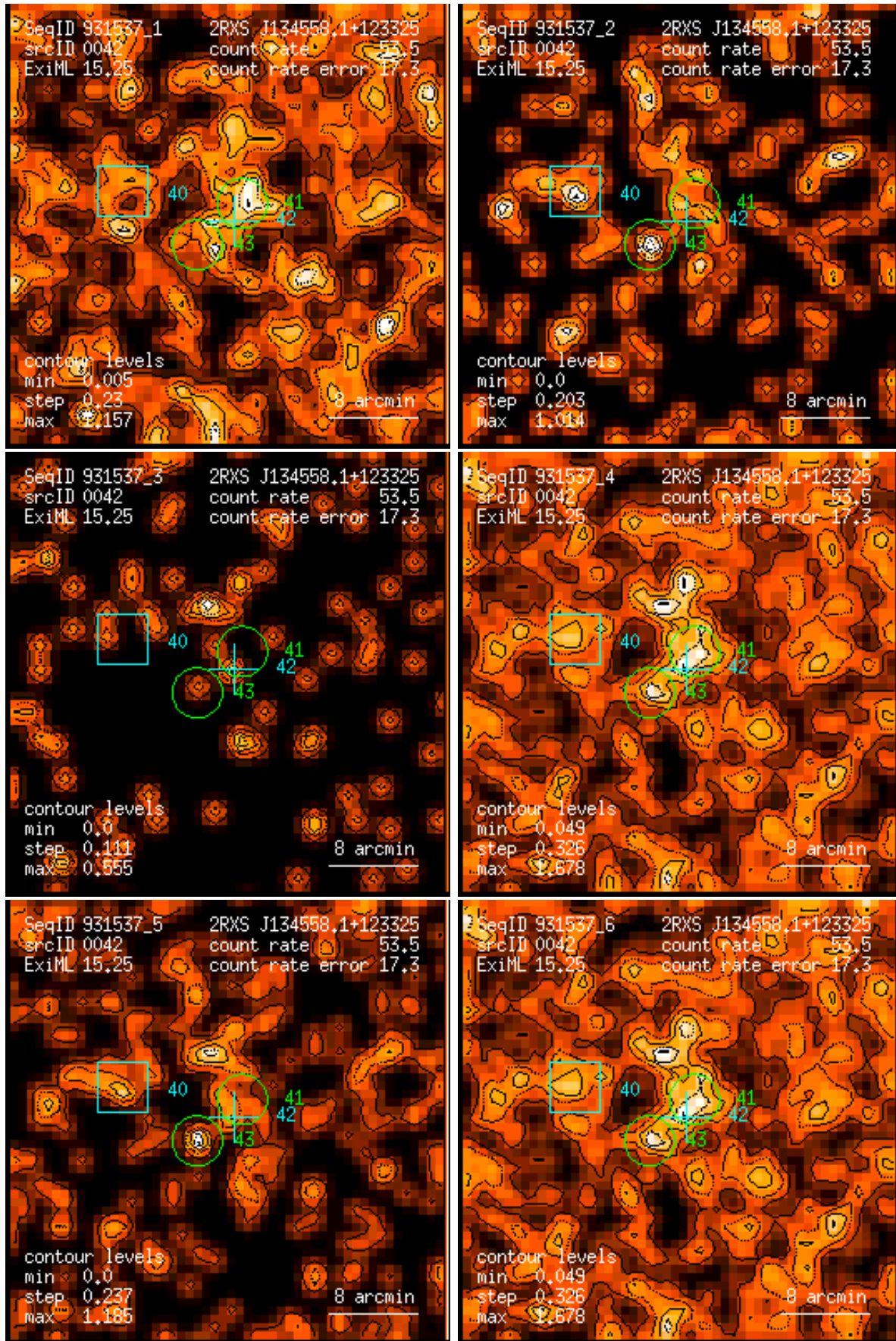
Figure 42: RASS 931537: detection 0042: band rate images, Gaussian filter: (1) PSPC channels 11 – 41, (2) 52 – 90, (3) 91 – 201, (4) 11 – 235, (5) 52 – 201, (6) 11 – 201. Broad band rates in counts/ks. Band rate contour levels in counts/ks/arcmin 2 .
