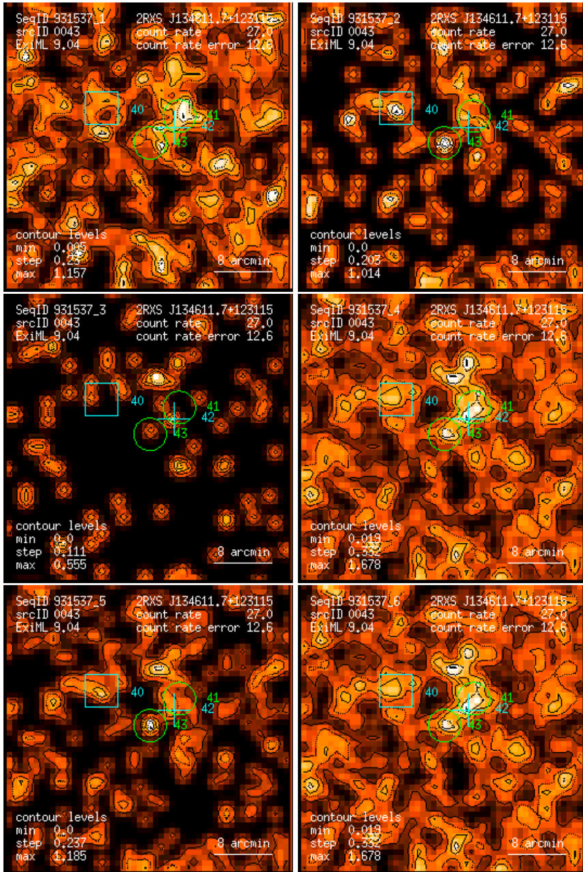
Figure 43: RASS 931537: detection 0043: band rate images, Gaussian filter: (1) PSPC channels 11 – 41, (2) 52 – 90, (3) 91 – 201, (4) 11 – 235, (5) 52 – 201, (6) 11 – 201. Broad band rates in counts/ks. Band rate contour levels in counts/ks/arcmin 2 .
