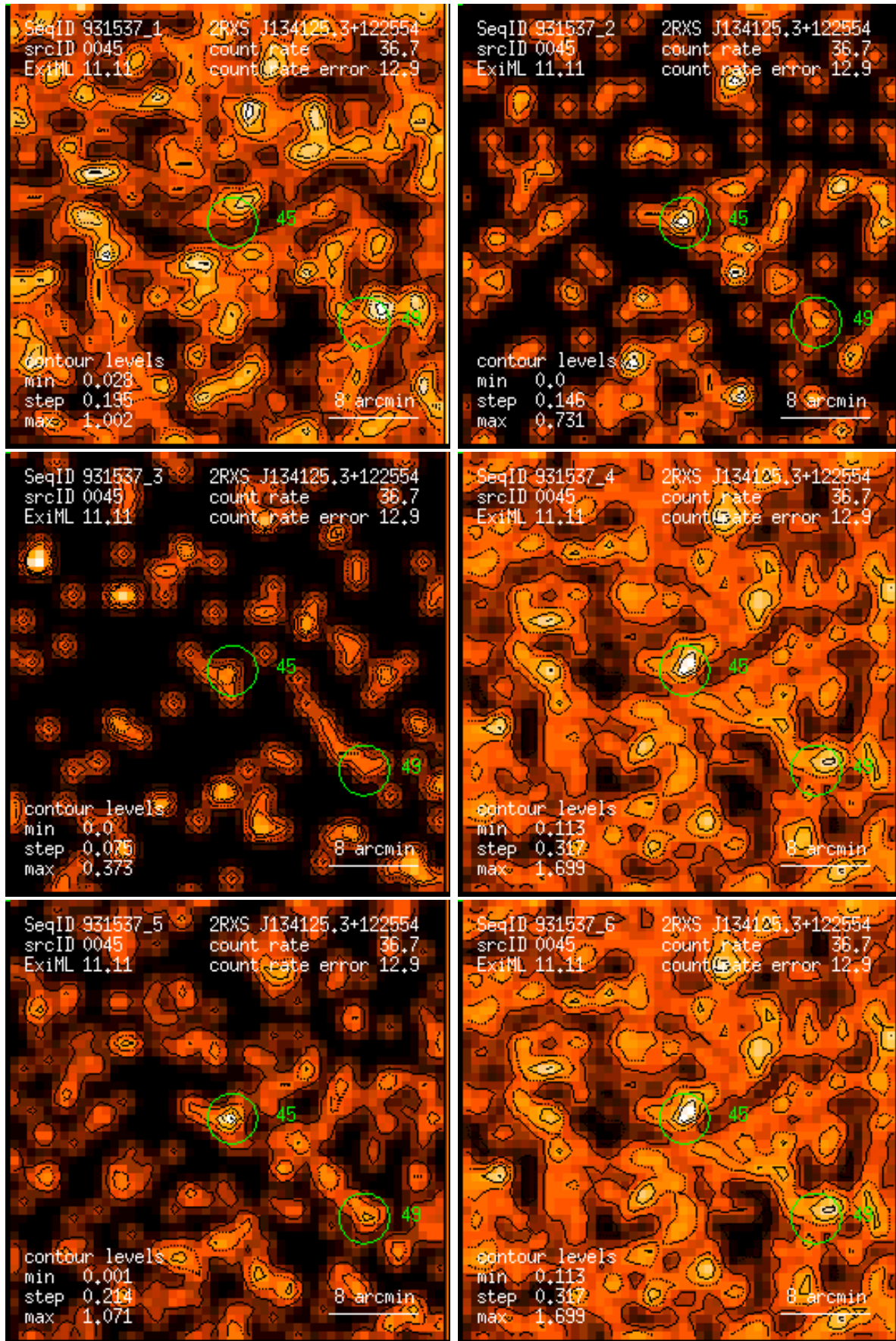
Figure 45: RASS 931537: detection 0045: band rate images, Gaussian filter: (1) PSPC channels 11 – 41, (2) 52 – 90, (3) 91 – 201, (4) 11 – 235, (5) 52 – 201, (6) 11 – 201. Broad band rates in counts/ks. Band rate contour levels in counts/ks/arcmin 2 .
