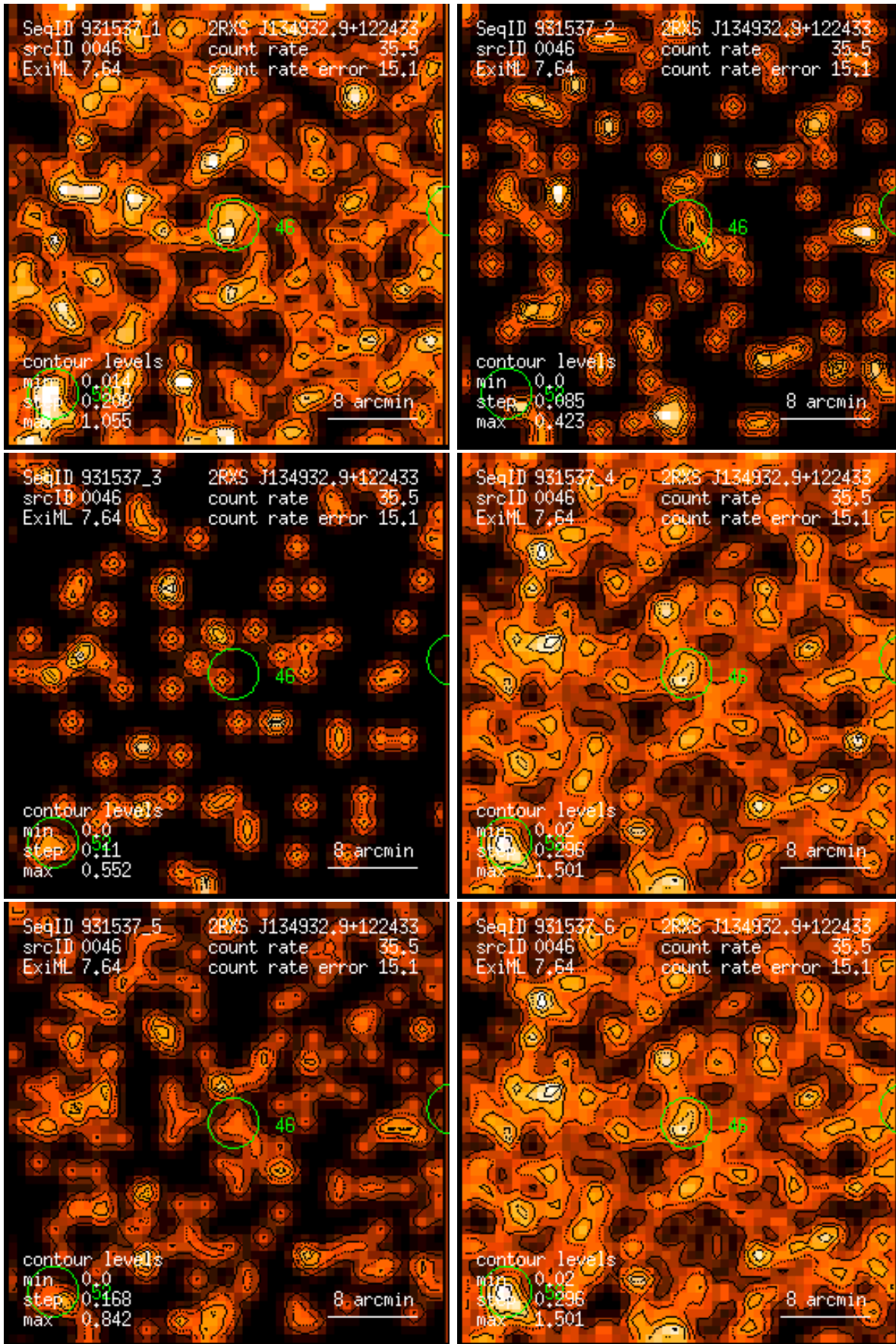
Figure 46: RASS 931537: detection 0046: band rate images, Gaussian filter: (1) PSPC channels 11 – 41, (2) 52 – 90, (3) 91 – 201, (4) 11 – 235, (5) 52 – 201, (6) 11 – 201. Broad band rates in counts/ks. Band rate contour levels in counts/ks/arcmin 2 .
