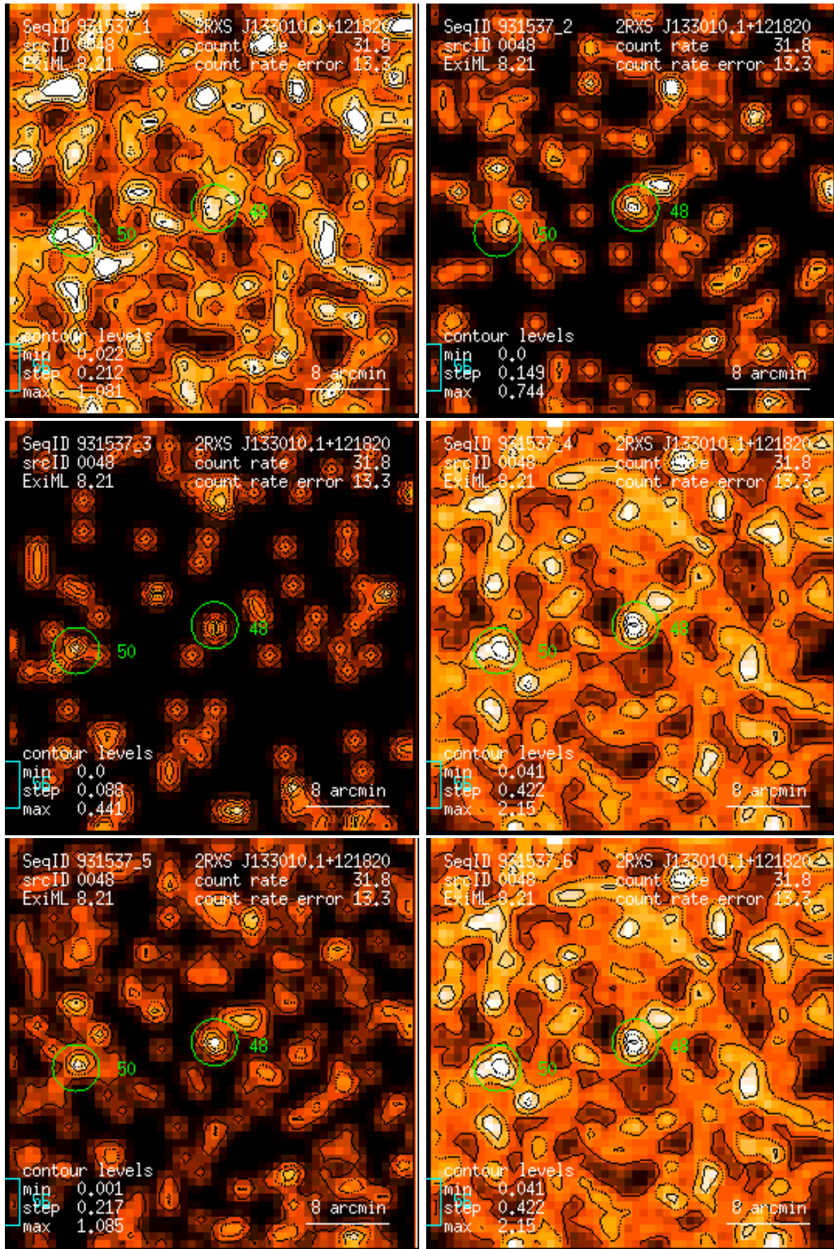
Figure 48: RASS 931537: detection 0048: band rate images, Gaussian filter: (1) PSPC channels 11 – 41, (2) 52 – 90, (3) 91 – 201, (4) 11 – 235, (5) 52 – 201, (6) 11 – 201. Broad band rates in counts/ks. Band rate contour levels in counts/ks/arcmin 2 .
