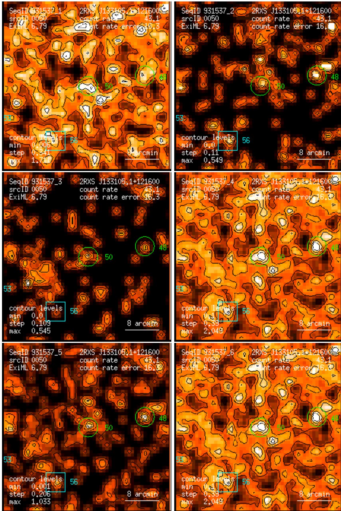
Figure 50: RASS 931537: detection 0050: band rate images, Gaussian filter: (1) PSPC channels 11 – 41, (2) 52 – 90, (3) 91 – 201, (4) 11 – 235, (5) 52 – 201, (6) 11 – 201. Broad band rates in counts/ks. Band rate contour levels in counts/ks/arcmin 2 .
