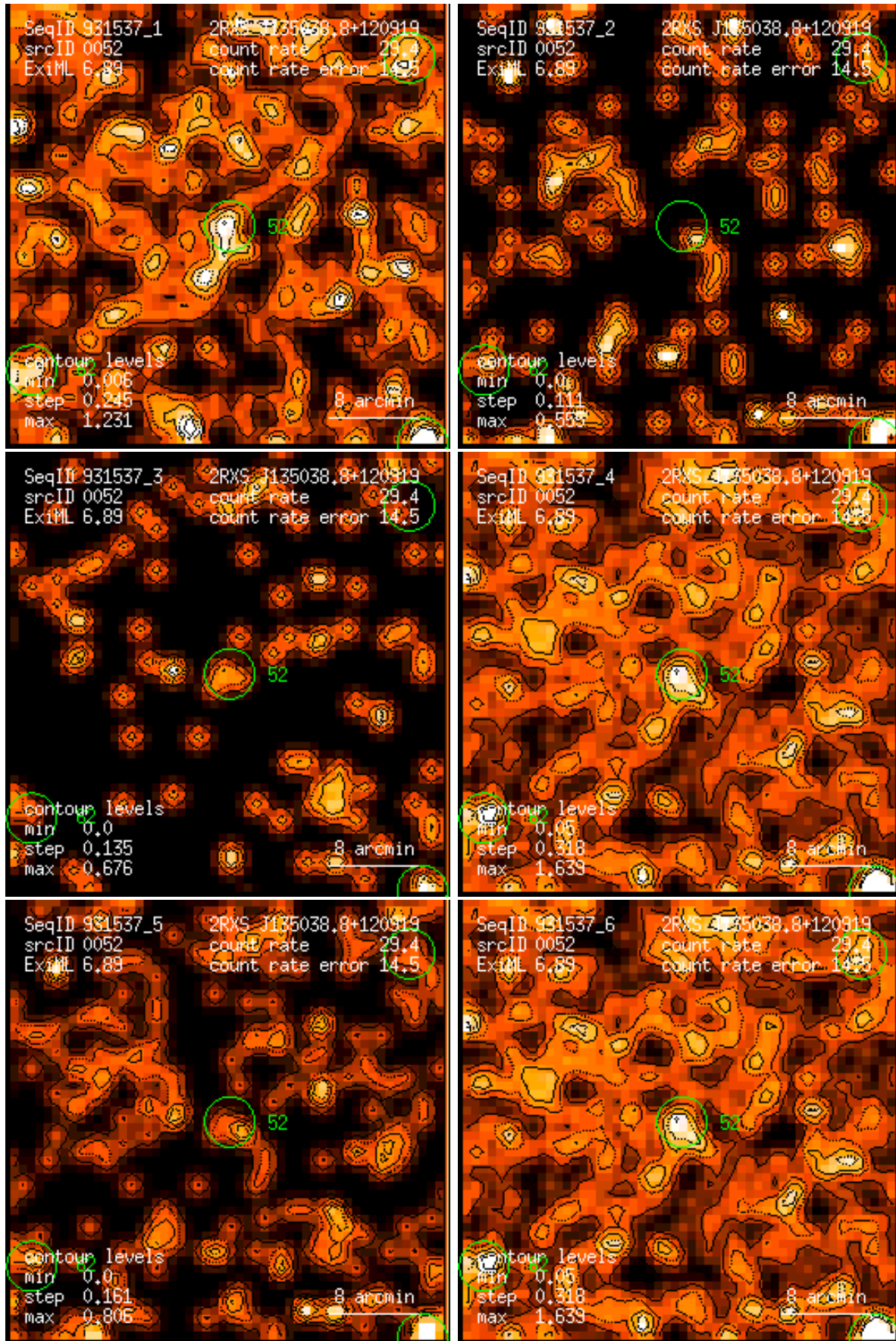
Figure 52: RASS 931537: detection 0052: band rate images, Gaussian filter: (1) PSPC channels 11 – 41, (2) 52 – 90, (3) 91 – 201, (4) 11 – 235, (5) 52 – 201, (6) 11 – 201. Broad band rates in counts/ks. Band rate contour levels in counts/ks/arcmin 2 .
