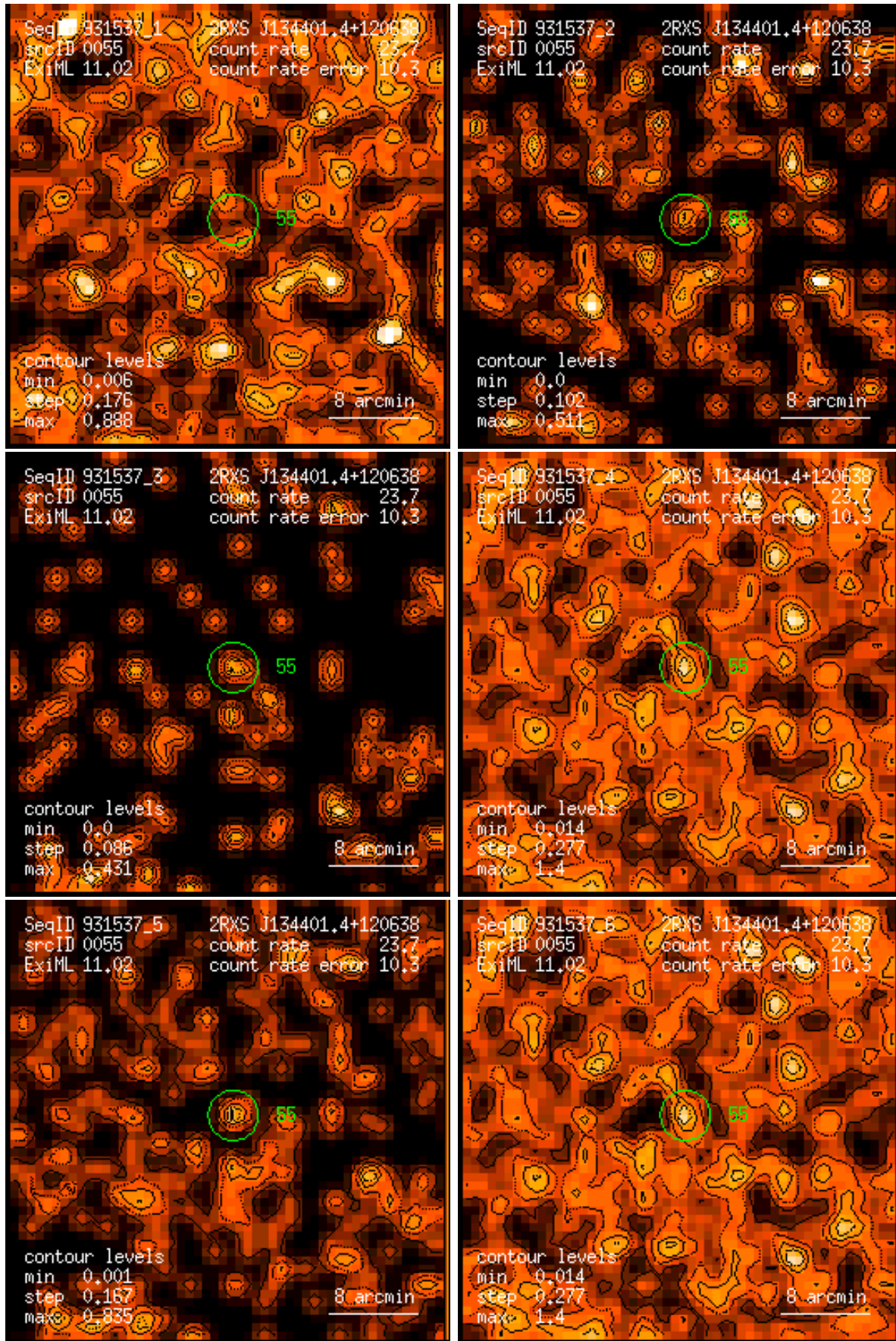
Figure 55: RASS 931537: detection 0055: band rate images, Gaussian filter: (1) PSPC channels 11 – 41, (2) 52 – 90, (3) 91 – 201, (4) 11 – 235, (5) 52 – 201, (6) 11 – 201. Broad band rates in counts/ks. Band rate contour levels in counts/ks/arcmin 2 .
