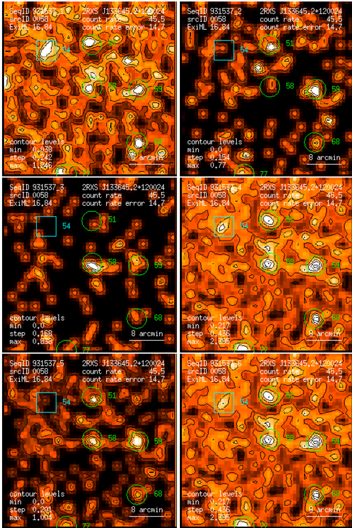
Figure 58: RASS 931537: detection 0058: band rate images, Gaussian filter: (1) PSPC channels 11 – 41, (2) 52 – 90, (3) 91 – 201, (4) 11 – 235, (5) 52 – 201, (6) 11 – 201. Broad band rates in counts/ks. Band rate contour levels in counts/ks/arcmin 2 .
