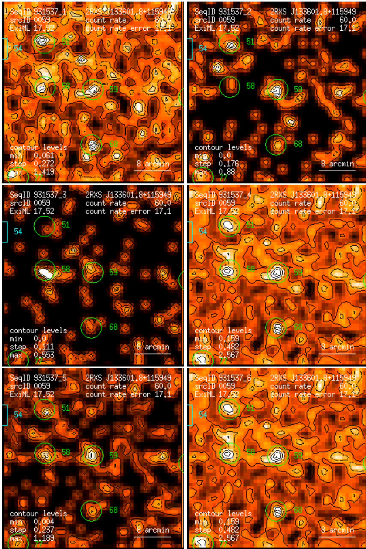
Figure 59: RASS 931537: detection 0059: band rate images, Gaussian filter: (1) PSPC channels 11 – 41, (2) 52 – 90, (3) 91 – 201, (4) 11 – 235, (5) 52 – 201, (6) 11 – 201. Broad band rates in counts/ks. Band rate contour levels in counts/ks/arcmin 2 .
