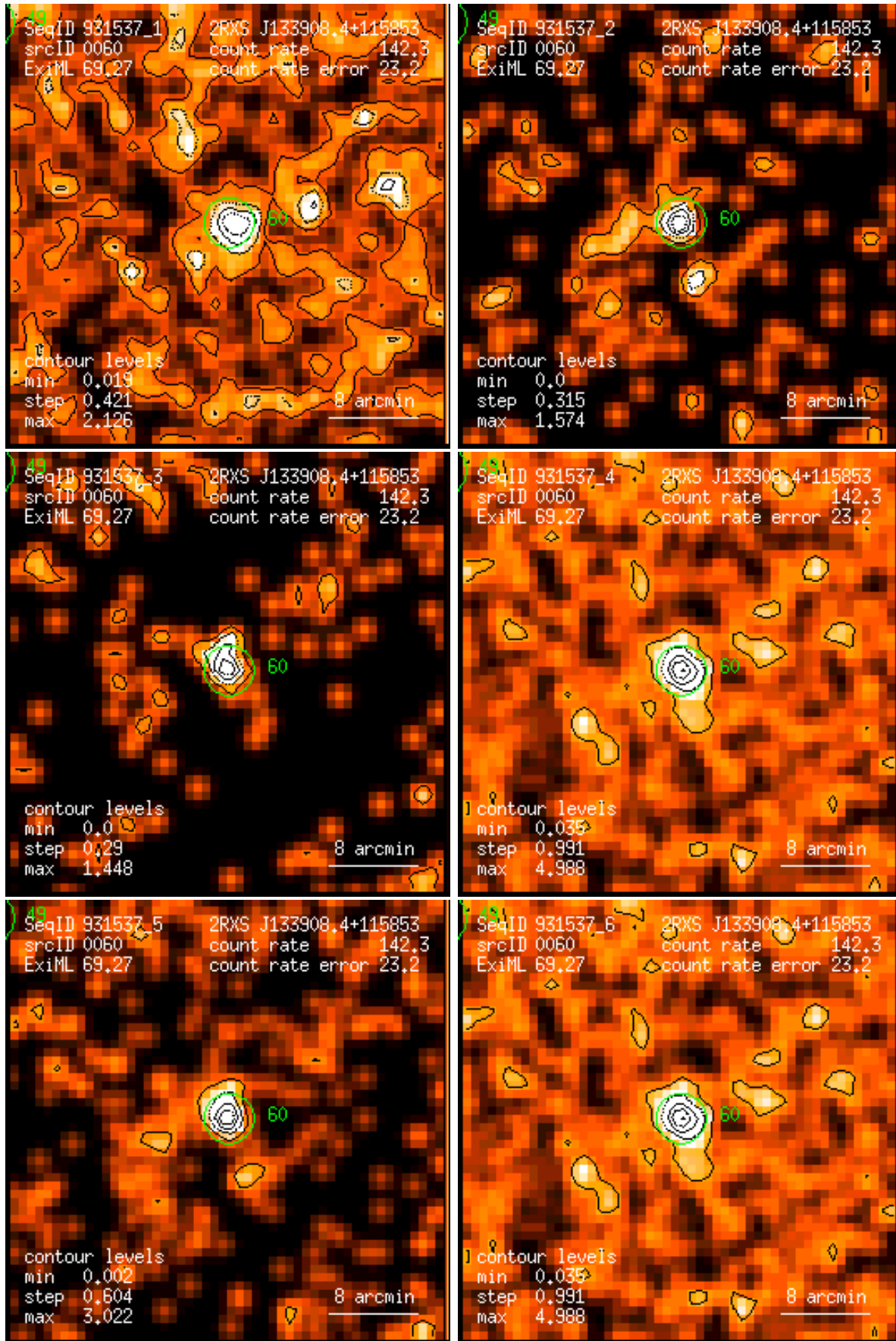
Figure 60: RASS 931537: detection 0060: band rate images, Gaussian filter: (1) PSPC channels 11 – 41, (2) 52 – 90, (3) 91 – 201, (4) 11 – 235, (5) 52 – 201, (6) 11 – 201. Broad band rates in counts/ks. Band rate contour levels in counts/ks/arcmin 2 .
