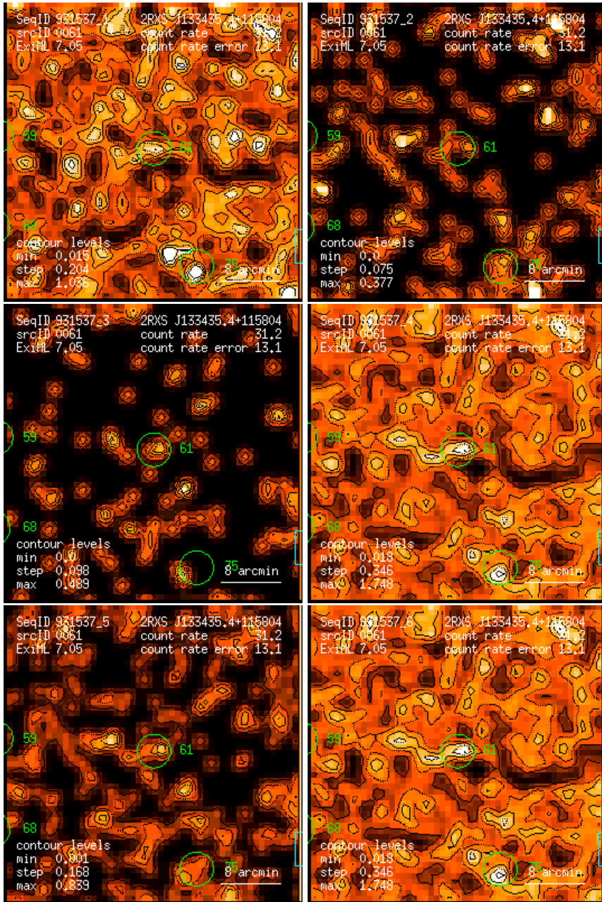
Figure 61: RASS 931537: detection 0061: band rate images, Gaussian filter: (1) PSPC channels 11 – 41, (2) 52 – 90, (3) 91 – 201, (4) 11 – 235, (5) 52 – 201, (6) 11 – 201. Broad band rates in counts/ks. Band rate contour levels in counts/ks/arcmin 2 .
