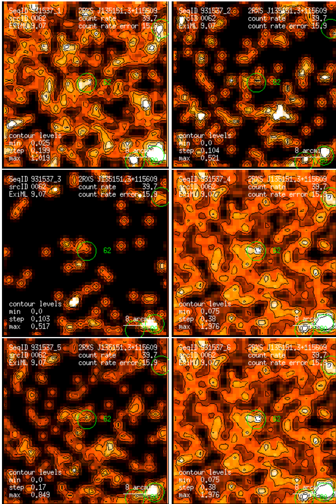
Figure 62: RASS 931537: detection 0062: band rate images, Gaussian filter: (1) PSPC channels 11 – 41, (2) 52 – 90, (3) 91 – 201, (4) 11 – 235, (5) 52 – 201, (6) 11 – 201. Broad band rates in counts/ks. Band rate contour levels in counts/ks/arcmin 2 .
