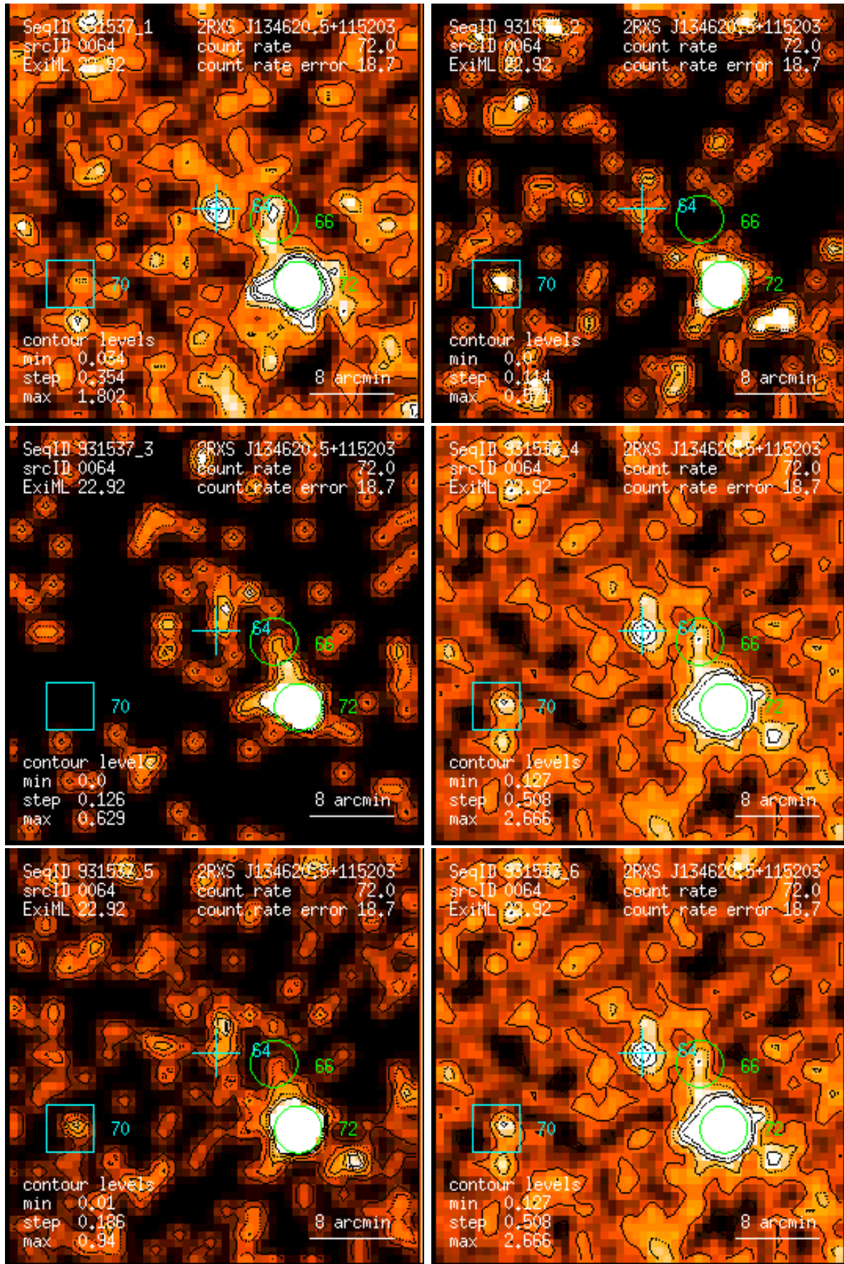
Figure 64: RASS 931537: detection 0064: band rate images, Gaussian filter: (1) PSPC channels 11 – 41, (2) 52 – 90, (3) 91 – 201, (4) 11 – 235, (5) 52 – 201, (6) 11 – 201. Broad band rates in counts/ks. Band rate contour levels in counts/ks/arcmin 2 .
