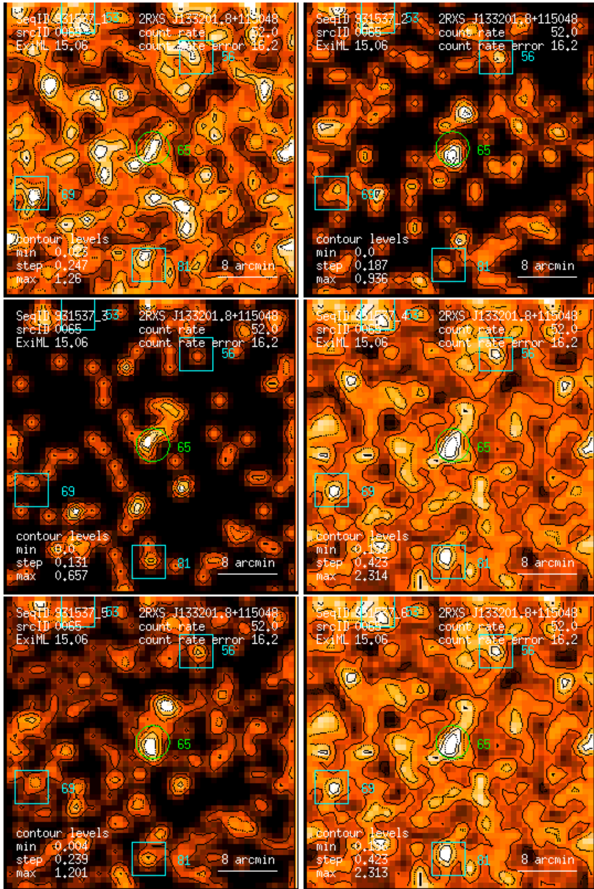
Figure 65: RASS 931537: detection 0065: band rate images, Gaussian filter: (1) PSPC channels 11 – 41, (2) 52 – 90, (3) 91 – 201, (4) 11 – 235, (5) 52 – 201, (6) 11 – 201. Broad band rates in counts/ks. Band rate contour levels in counts/ks/arcmin 2 .
