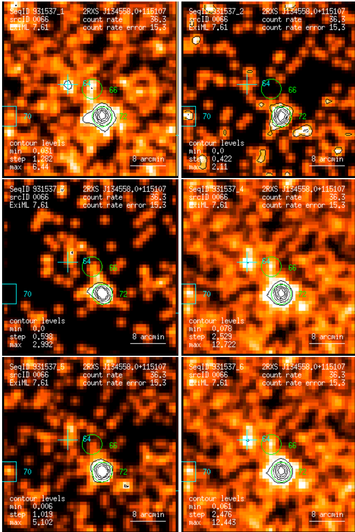
Figure 66: RASS 931537: detection 0066: band rate images, Gaussian filter: (1) PSPC channels 11 – 41, (2) 52 – 90, (3) 91 – 201, (4) 11 – 235, (5) 52 – 201, (6) 11 – 201. Broad band rates in counts/ks. Band rate contour levels in counts/ks/arcmin 2 .
