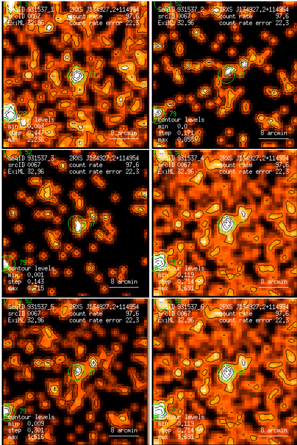
Figure 67: RASS 931537: detection 0067: band rate images, Gaussian filter: (1) PSPC channels 11 – 41, (2) 52 – 90, (3) 91 – 201, (4) 11 – 235, (5) 52 – 201, (6) 11 – 201. Broad band rates in counts/ks. Band rate contour levels in counts/ks/arcmin 2 .
