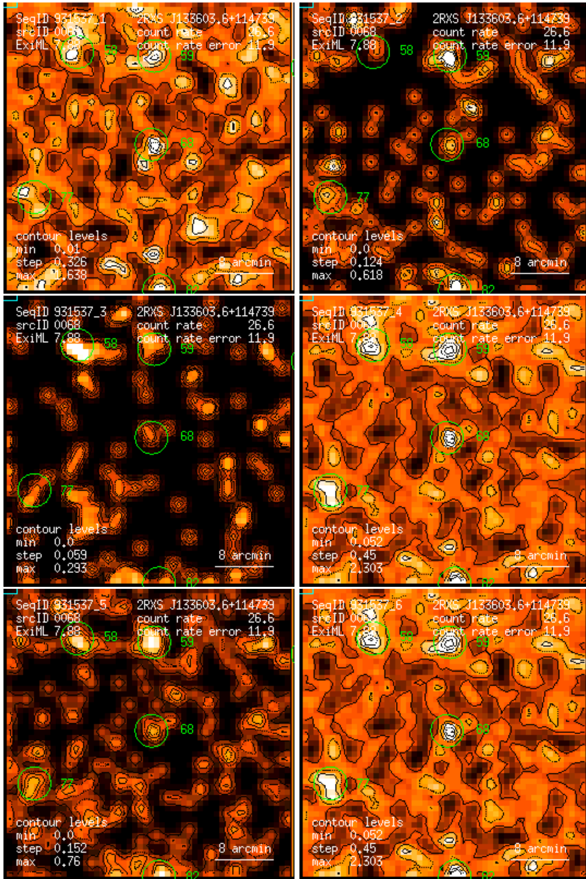
Figure 68: RASS 931537: detection 0068: band rate images, Gaussian filter: (1) PSPC channels 11 – 41, (2) 52 – 90, (3) 91 – 201, (4) 11 – 235, (5) 52 – 201, (6) 11 – 201. Broad band rates in counts/ks. Band rate contour levels in counts/ks/arcmin 2 .
