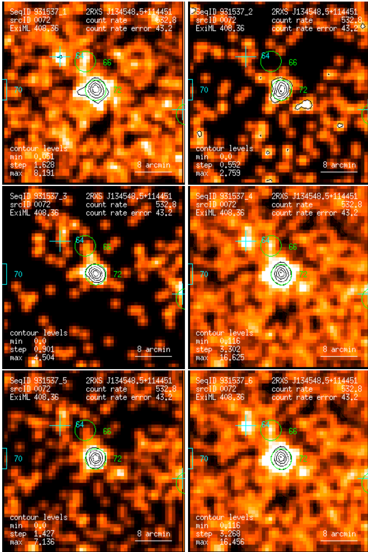
Figure 72: RASS 931537: detection 0072: band rate images, Gaussian filter: (1) PSPC channels 11 – 41, (2) 52 – 90, (3) 91 – 201, (4) 11 – 235, (5) 52 – 201, (6) 11 – 201. Broad band rates in counts/ks. Band rate contour levels in counts/ks/arcmin 2 .
