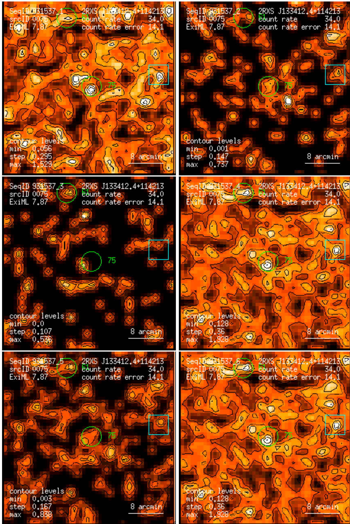
Figure 75: RASS 931537: detection 0075: band rate images, Gaussian filter: (1) PSPC channels 11 – 41, (2) 52 – 90, (3) 91 – 201, (4) 11 – 235, (5) 52 – 201, (6) 11 – 201. Broad band rates in counts/ks. Band rate contour levels in counts/ks/arcmin 2 .
