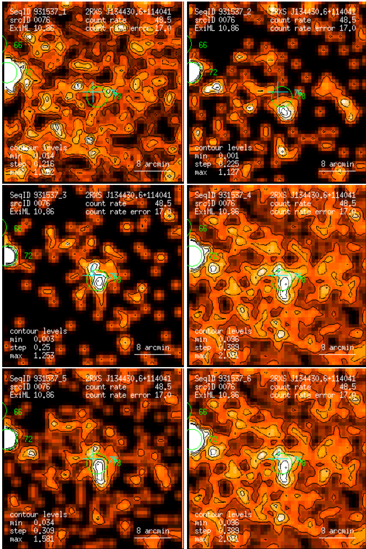
Figure 76: RASS 931537: detection 0076: band rate images, Gaussian filter: (1) PSPC channels 11 – 41, (2) 52 – 90, (3) 91 – 201, (4) 11 – 235, (5) 52 – 201, (6) 11 – 201. Broad band rates in counts/ks. Band rate contour levels in counts/ks/arcmin 2 .
