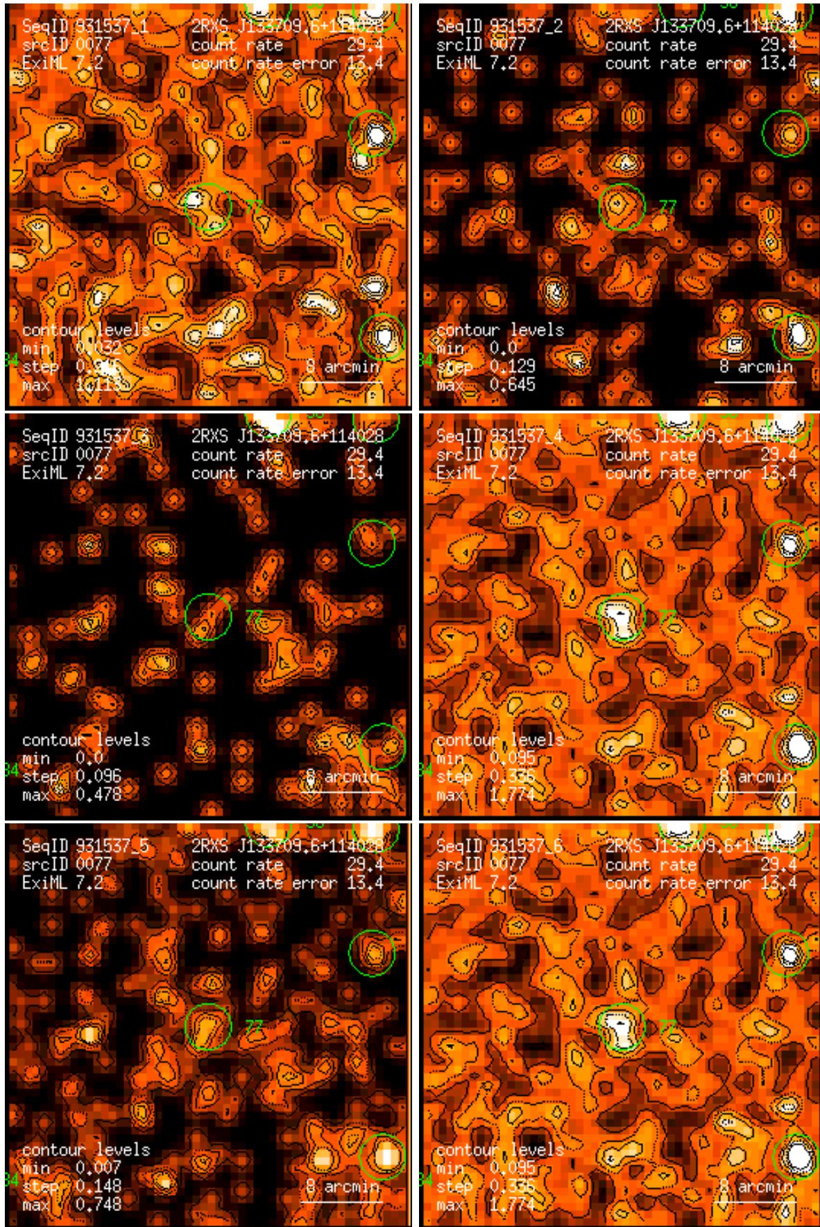
Figure 77: RASS 931537: detection 0077: band rate images, Gaussian filter: (1) PSPC channels 11 – 41, (2) 52 – 90, (3) 91 – 201, (4) 11 – 235, (5) 52 – 201, (6) 11 – 201. Broad band rates in counts/ks. Band rate contour levels in counts/ks/arcmin 2 .
